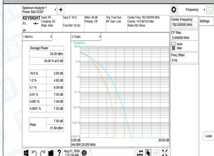
Band13-5MHz-16QAM-23255-1RB#0-PASS
