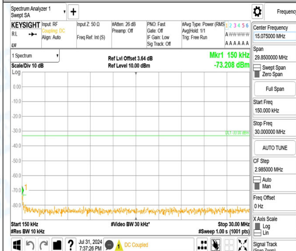
Band2_20MHz_16QAM_18700_1RB#0_0.15~30_0.15~30
