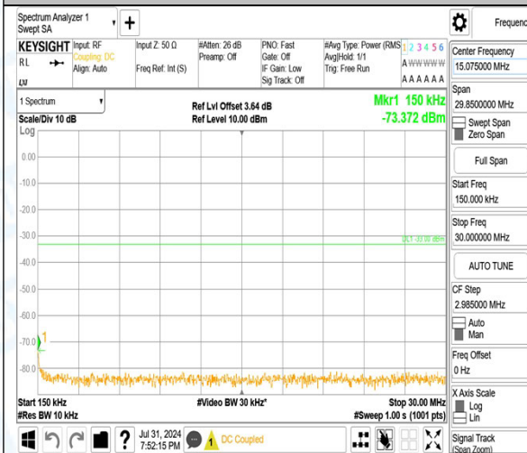
Band2_20MHz_QPSK_18900_100RB#0_0.15~30_0.15~30
