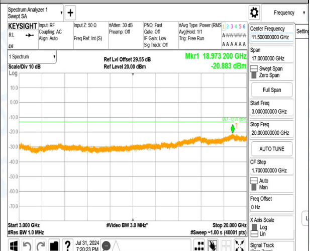
Band2_20MHz_QPSK_18700_1RB#0_0.15~30_0.15~30
