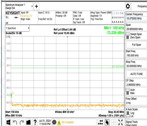
Band2_15MHz_16QAM_19125_1RB#74_0.15~30_0.15~30
