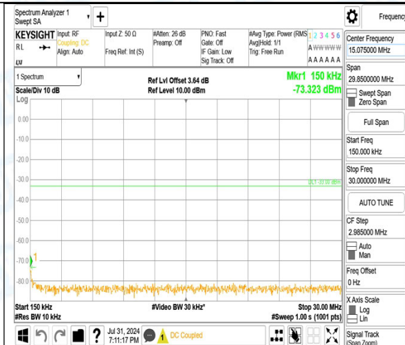
Band2_15MHz_16QAM_18675_1RB#74_1000~3000_1000~3000
