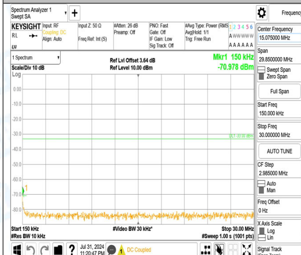
Band4_15MHz_16QAM_20175_1RB#74_0.15~30_0.15~30
