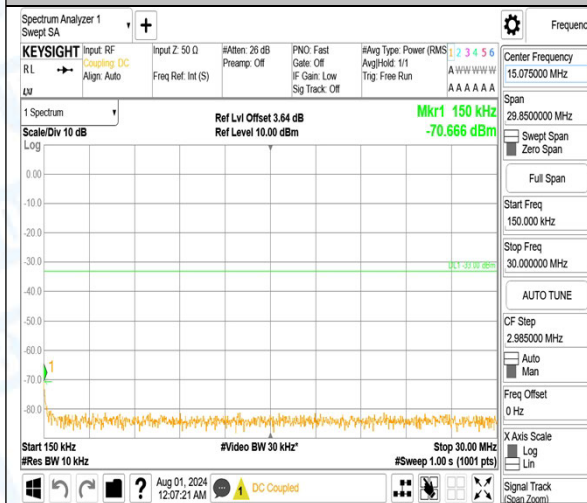
Band4_20MHz_QPSK_20175_100RB#0_0.15~30_0.15~30
