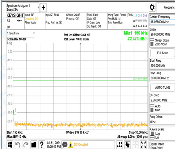
Band4_15MHz_16QAM_20325_1RB#74_0.15~30_0.15~30
