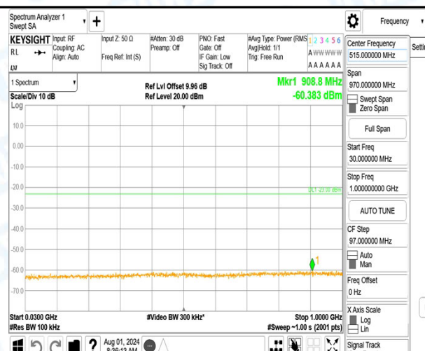
Band66_1.4MHz_QPSK_132665_1RB#5_3000~20000_3000~20000
