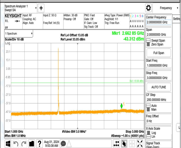
Band66_5MHz_QPSK_131997_1RB#0_1000~3000_1000~3000
