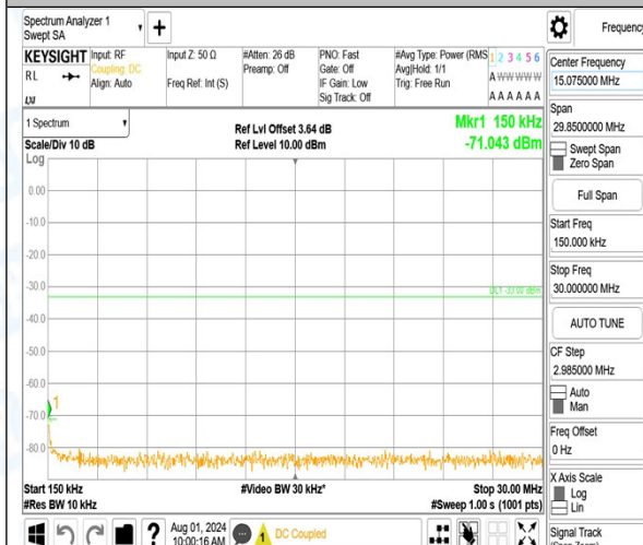
Band66_5MHz_QPSK_132322_1RB#0_0.15~30_0.15~30
