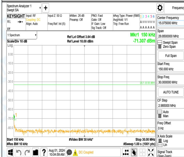
Band66_5MHz_QPSK_132322_25RB#0_0.15~30_0.15~30
