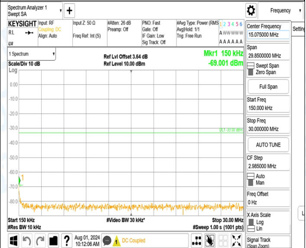
Band66_5MHz_QPSK_132647_25RB#0_1000~3000_1000~3000
