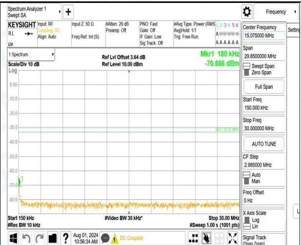
Band66_10MHz_16QAM_132322_1RB#49_1000~3000_1000~3000
