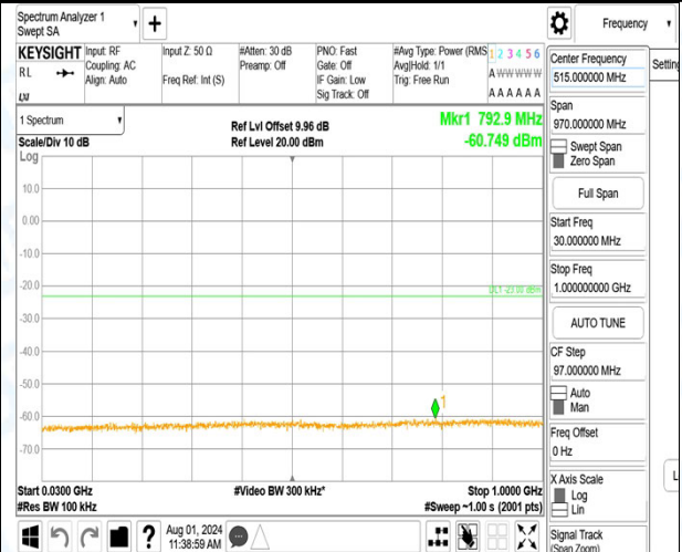
Band66_15MHz_QPSK_132322_1RB#74_3000~20000_3000~20
