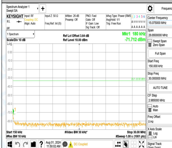
Band66_15MHz_QPSK_132597_75RB#0_1000~3000_1000~3000
