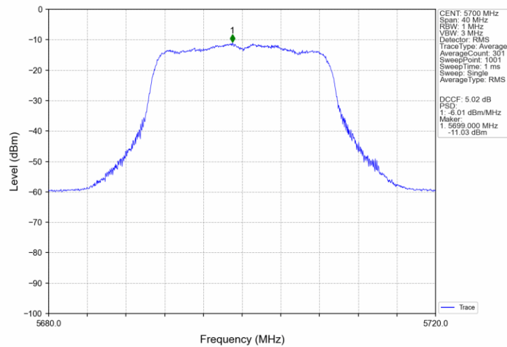
802.11ac(VHT20)_HCH_5700MHz_Ant2_NTNV
