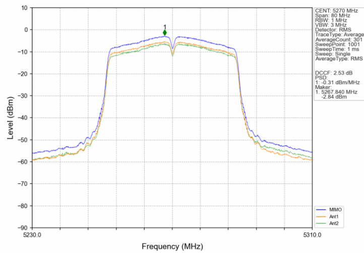
802.11ac(VHT40)_LCH_5270MHz_MIMO_NTNV
