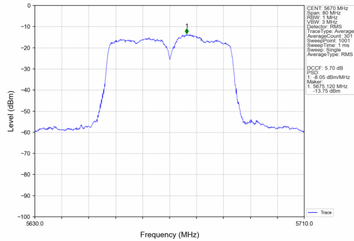
802.11ac(VHT40)_HCH_5670MHz_MIMO_NTNV
