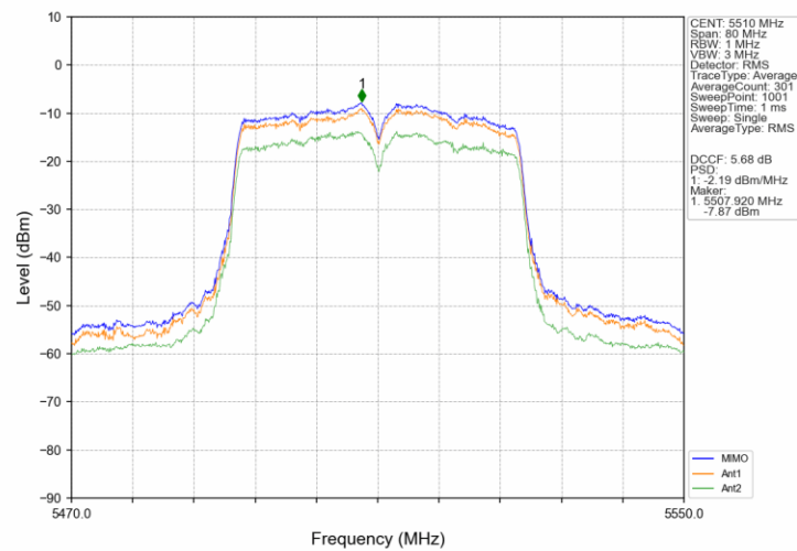
802.11ac(VHT40)_LCH_5510MHz_MIMO_NTNV
