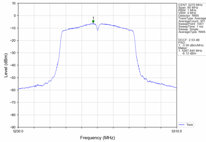
802.11ac(VHT40)_LCH_5270MHz_MIMO_NTNV
