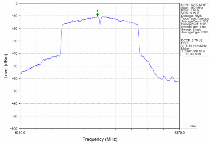
802.11ac(VHT80)_MCH_5290MHz_MIMO_NTNV
