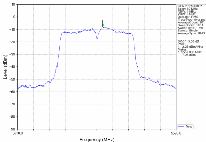
802.11ac(VHT40)_MCH_5550MHz_Ant2_NTNV
