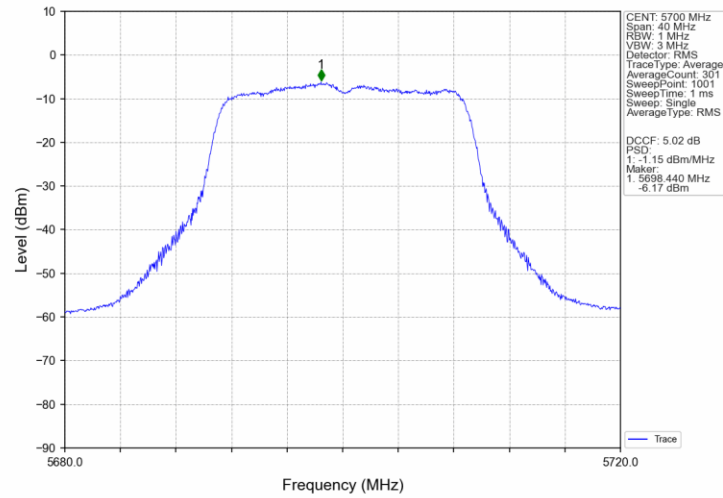
802.11ac(VHT20)_HCH_5700MHz_Ant2_NTNV
