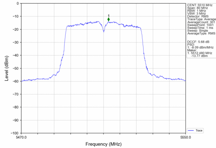
802.11ac(VHT40)_LCH_5510MHz_MIMO_NTNV
