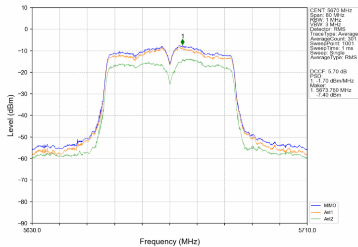
802.11ac(VHT40)_HCH_5670MHz_MIMO_NTNV
