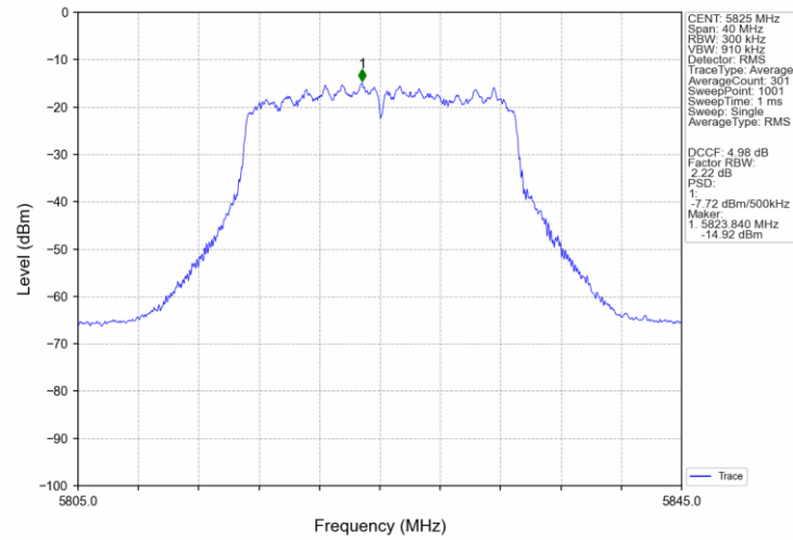
802.11ac(VHT20)_HCH_5825MHz_MIMO_NTNV
