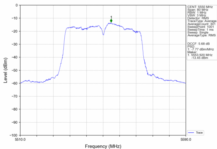
802.11ac(VHT40)_MCH_5550MHz_Ant2_NTNV
