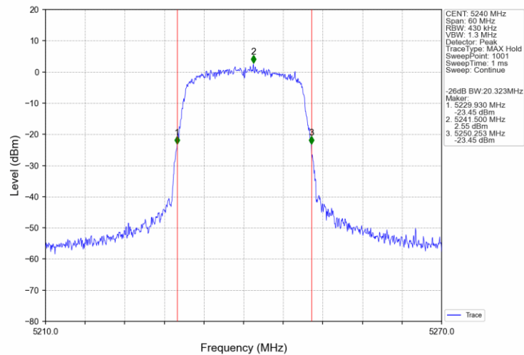
802.11ac(VHT20)_HCH_5240MHz_Ant0_NTNV
