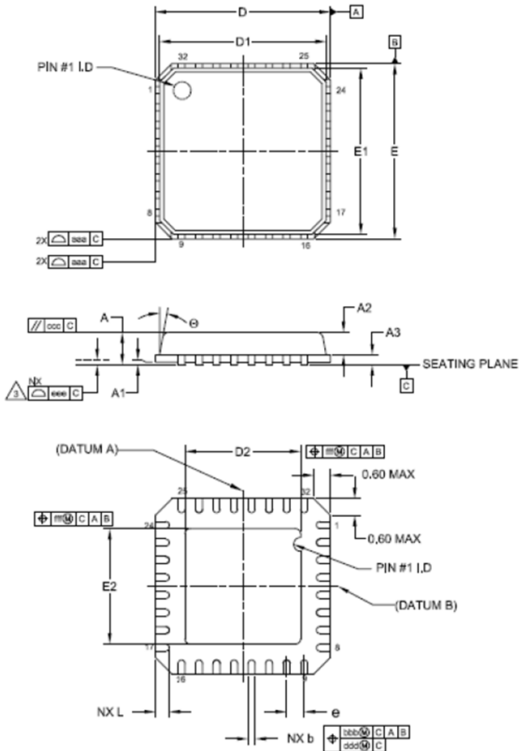
Figure 6 - QFN32 - Outline
