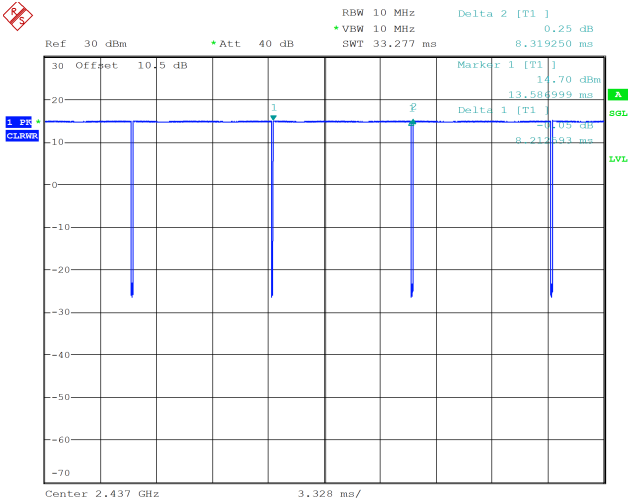
b_2437MHz_Chain 0 8.213 ms,8.319ms
