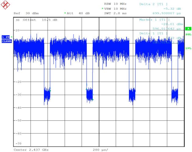
n20_2437MHz_Chain 0 0.601 ms,0.7ms
