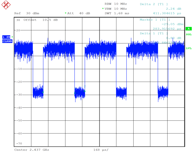
n40_2437MHz_Chain 0 0.313 ms,0.41ms
