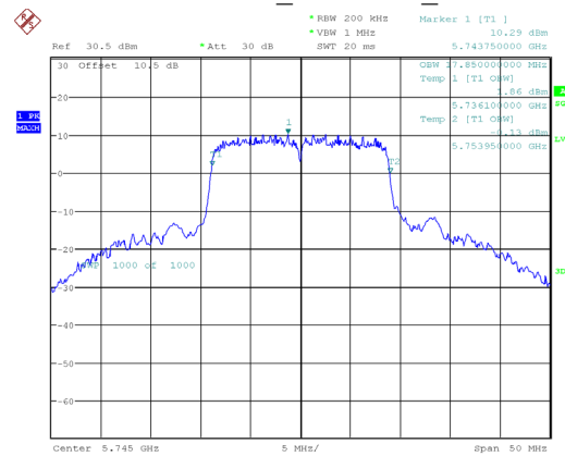
802.11ac20_5745MHz_Chain 1
