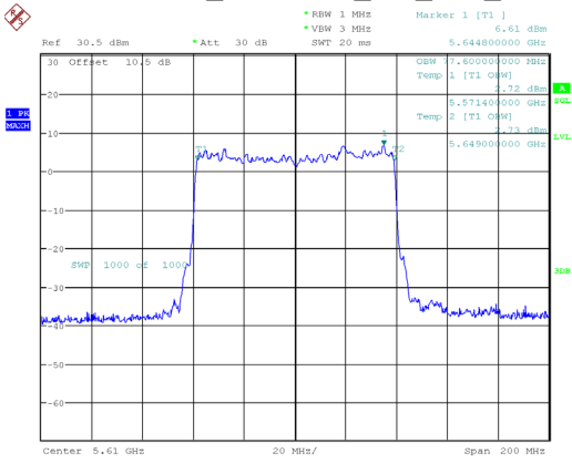
802.11ax80_5610MHz_RU_Full_Chain 1
