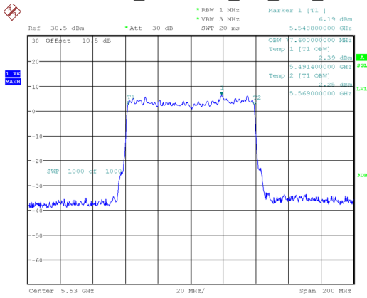
802.11ax80_5530MHz_RU_Full_Chain 1
