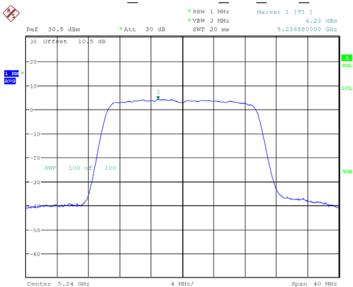
802.11ax20_5240MHz_RU_Full_Chain 0
