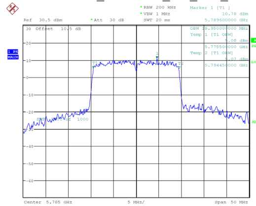
802.11ax20_5785MHz_RU_Full_Chain 0
