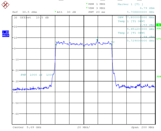
802.11ax80_5690MHz_RU_Full_Chain 1
