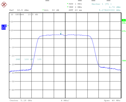
802.11ax20_5180MHz_RU_Full_Chain 0
