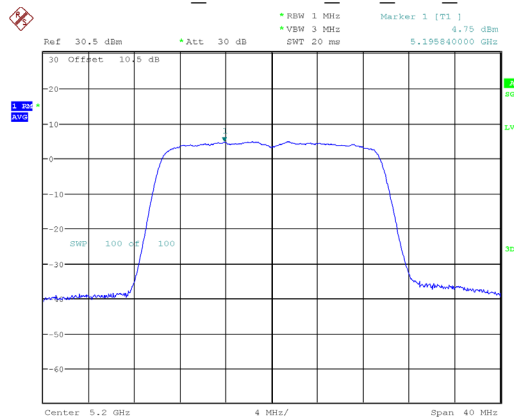
802.11ax20_5200MHz_RU_Full_Chain 0
