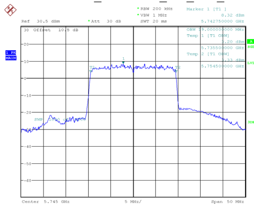
802.11ax20_5745MHz_RU_Full_Chain 1
