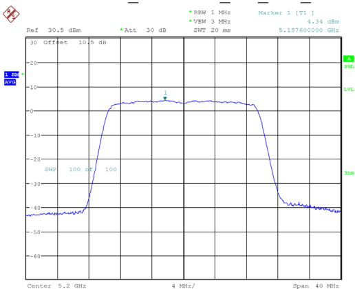
802.11ax20_5200MHz_RU_Full_Chain 1
