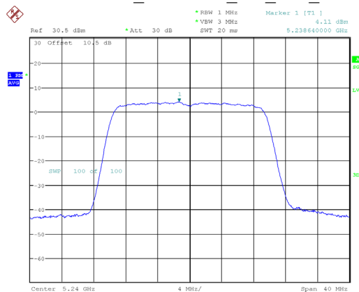
802.11ax20_5240MHz_RU_Full_Chain 1
