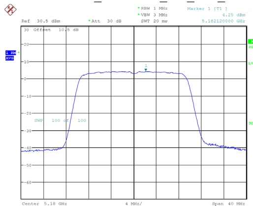
802.11ax20_5180MHz_RU_Full_Chain 1
