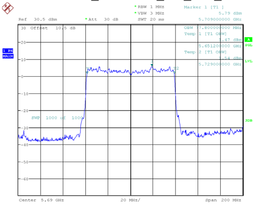
802.11ax80_5690MHz_RU_Full_Chain 0
