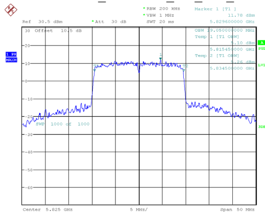
802.11ax20_5825MHz_RU_Full_Chain 1
