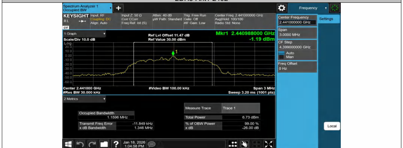
2DH5-Ant1-2441
