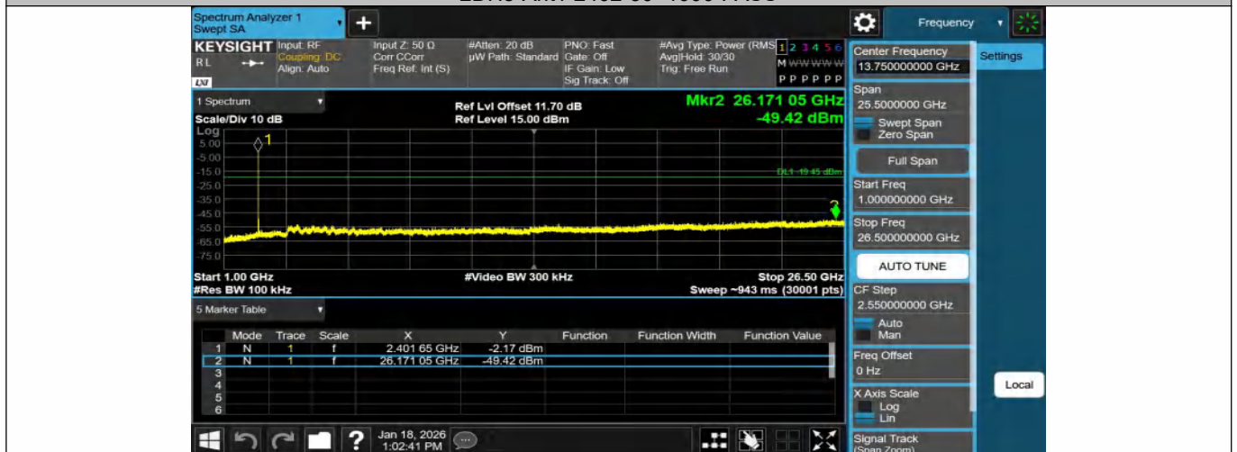
2DH5-Ant1-2402-1000~26500-PASS
