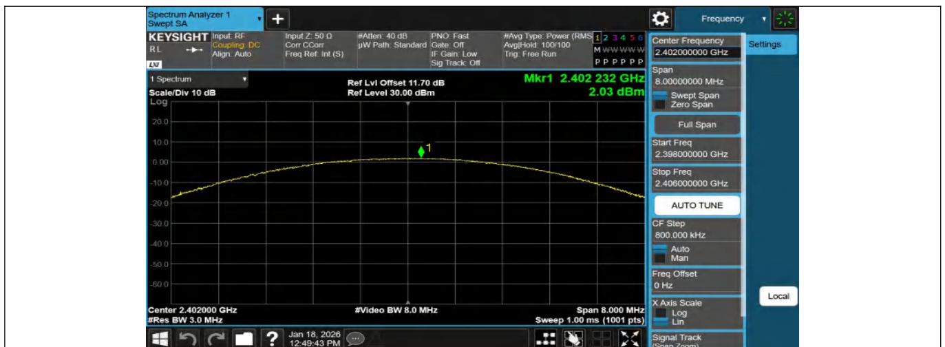
2DH5-Ant1-2402-PASS
