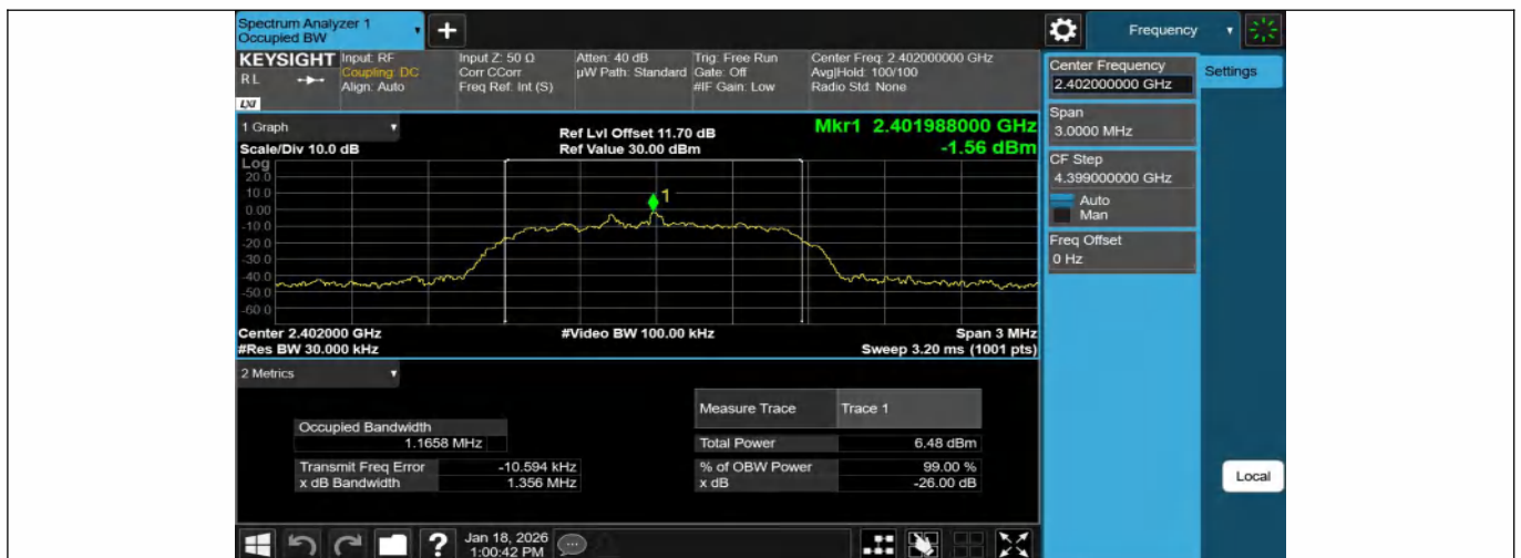
2DH5-Ant1-2402
