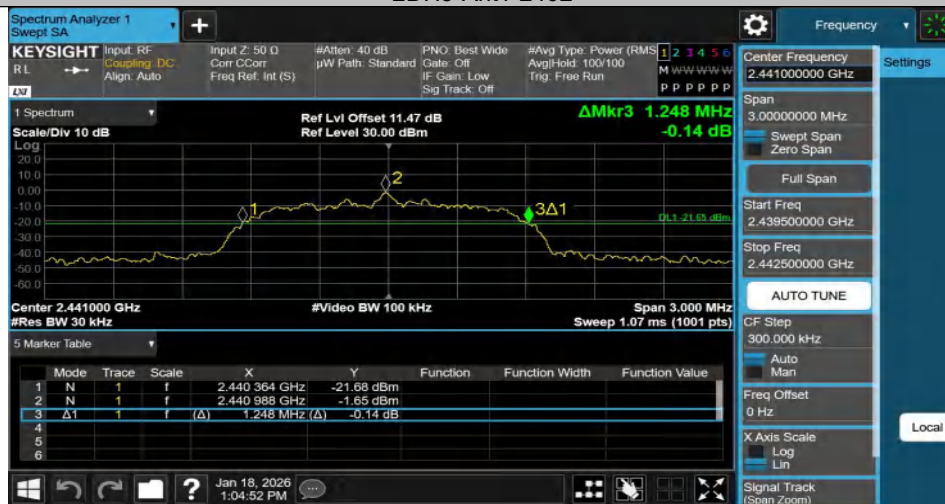
2DH5-Ant1-2441
