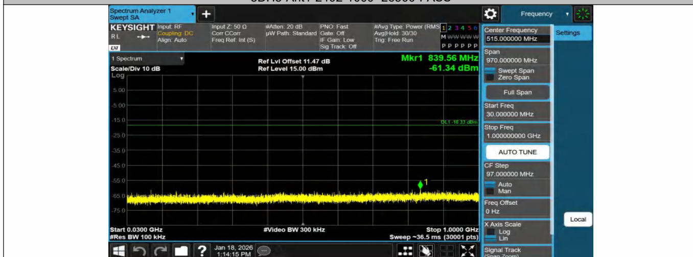
3DH5-Ant1-2441-30~1000-PASS
