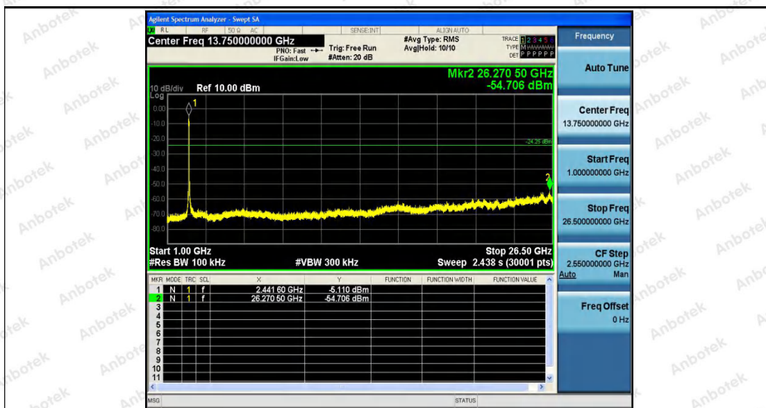
11N40_Ant1_2452_0~Reference
