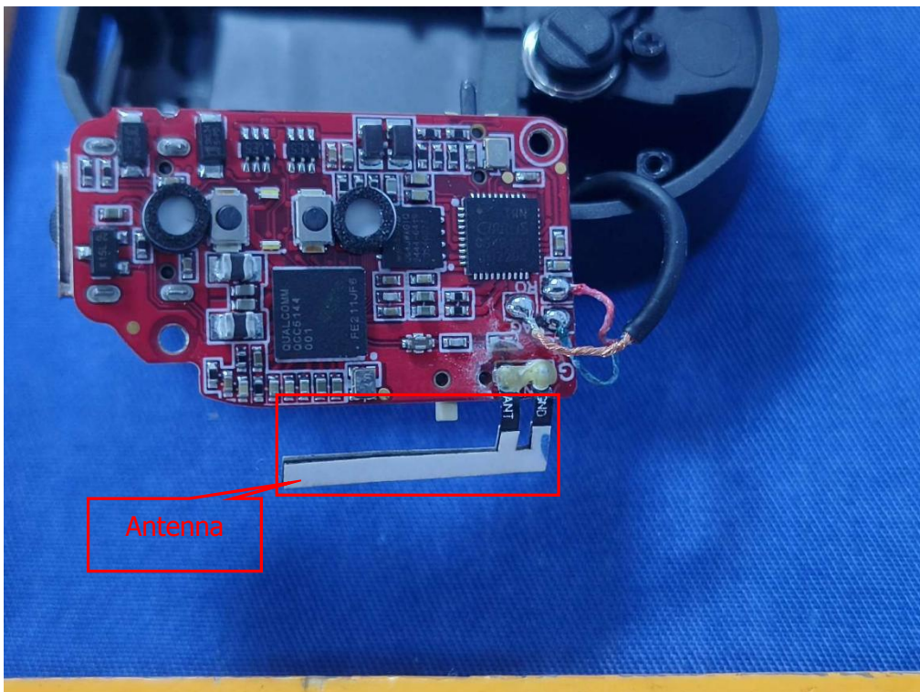
Internal view of unit (Model:UP TRAVEL)
