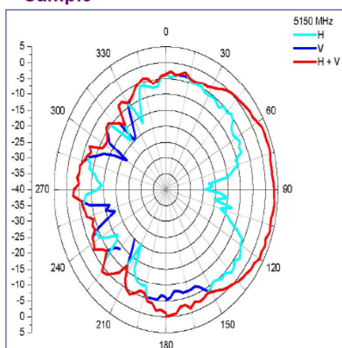
Radiated Pattern diagram for Antenna Gain
