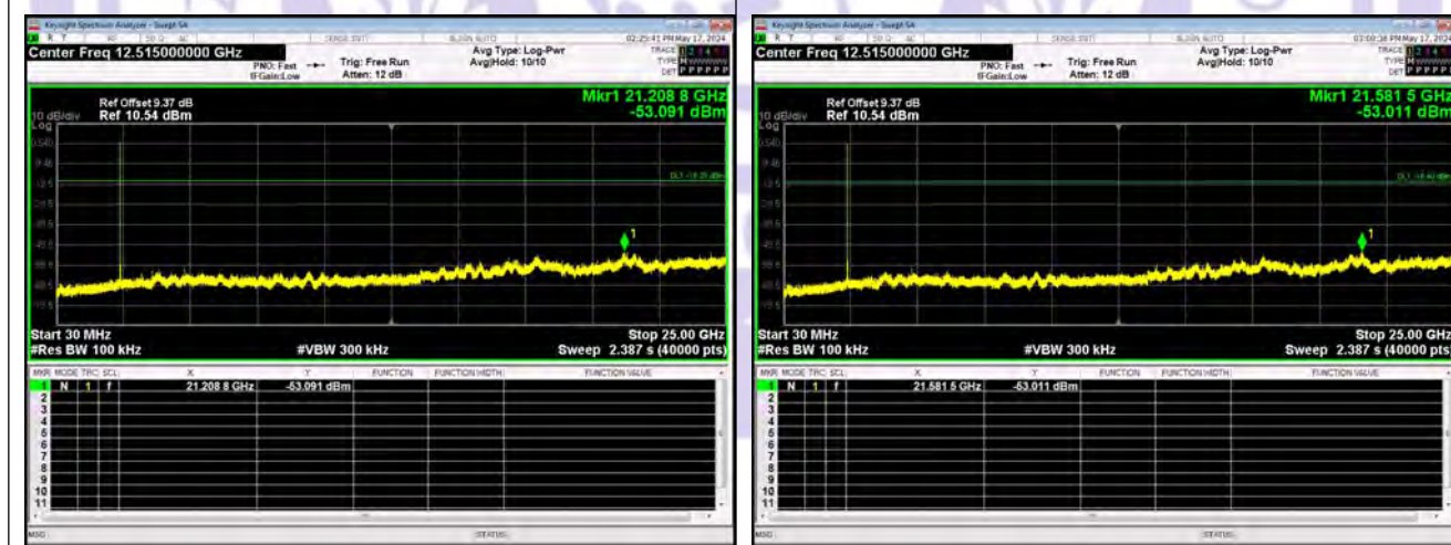
Spurious Emission
