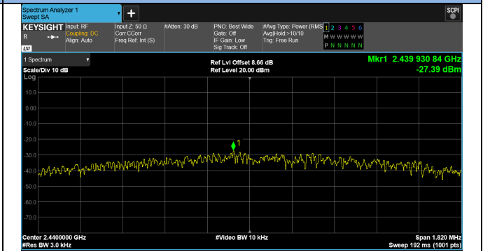
RF PHY 2Mbps 2440MHz
