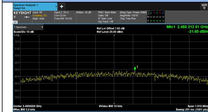
RF PHY 2Mbps 2480MHz
