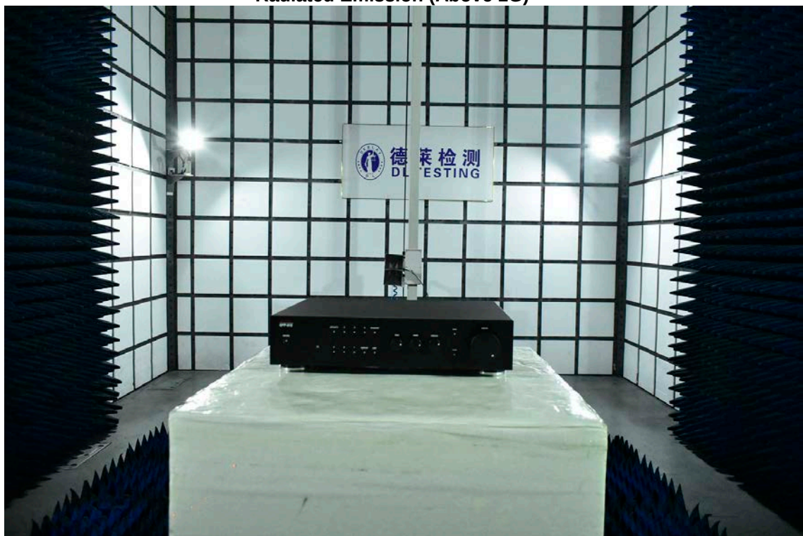
Radiated Emission (Above 1G)
