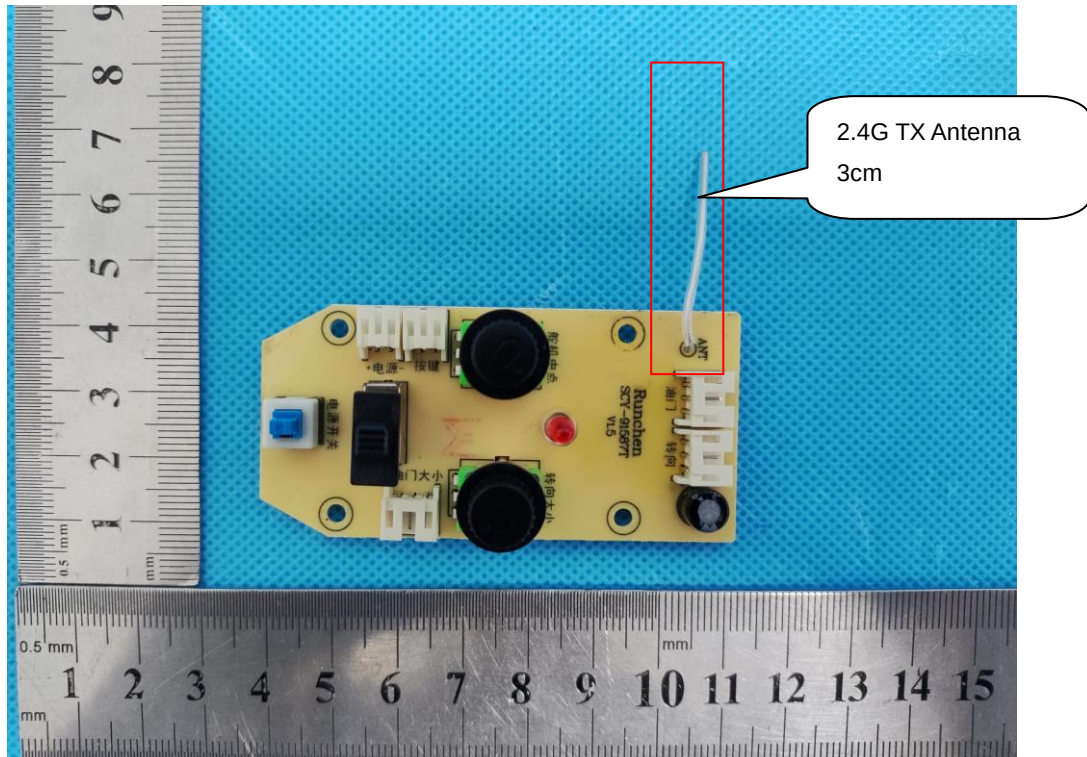
INTERNAL VIEW-5 OF EUT
