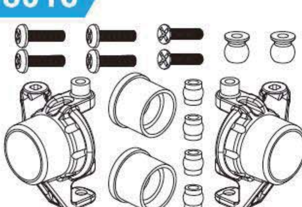
金属前转向节组件(L+R) Metal front steering knuckle assembly (L+R)
