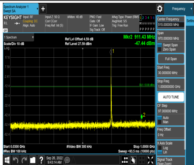
Band17-5MHz-QPSK-23790-1RB#0-Range1:30~1000MHz
