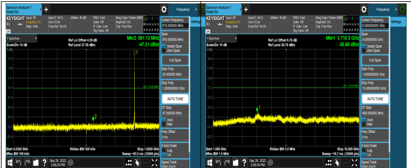
Band26-1.4MHz-QPSK-27033-1RB#0-Range1:30~1000MHz
