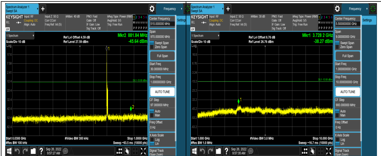
Band26-1.4MHz-QPSK-26697-1RB#0-Range1:30~1000MHz
