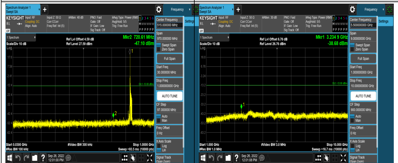
Band26-15MHz-QPSK-26965-1RB#0-Range1:30~1000MHz
