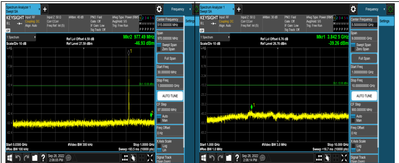
Band26-1.4MHz-16QAM-26915-1RB#0-Range1:30 ~1000MHz
