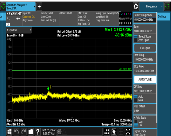
Band17-5MHz-QPSK-23755-1RB#0-Range2:1000~10000MHz
