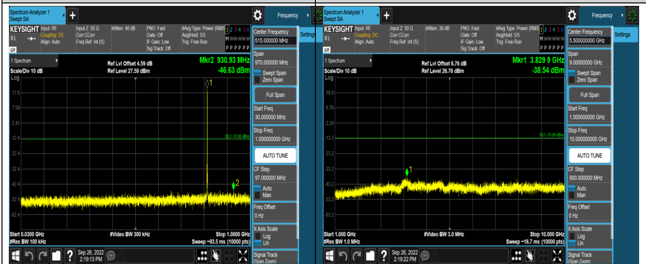
Band26-1.4MHz-QPSK-26740-1RB#0-Range1:30~1000MHz
