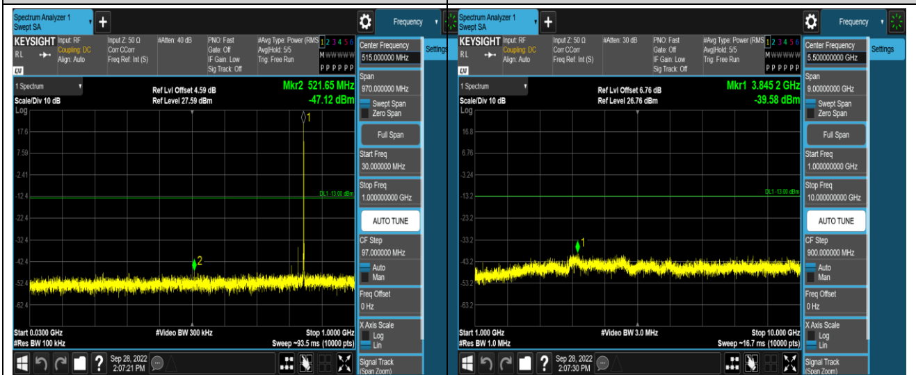
Band26-1.4MHz-16QAM-27033-1RB#0-Range1:30 ~1000MHz
