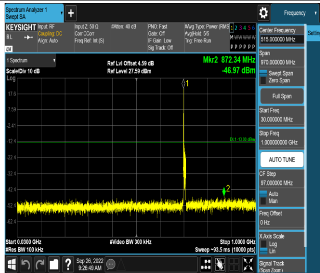
Band17-5MHz-QPSK-23755-1RB#0-Range1:30~1000MHz
