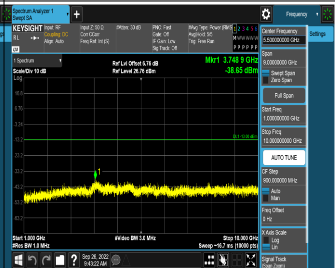
Band17-5MHz-QPSK-23790-1RB#0-Range2:1000~10000MHz
