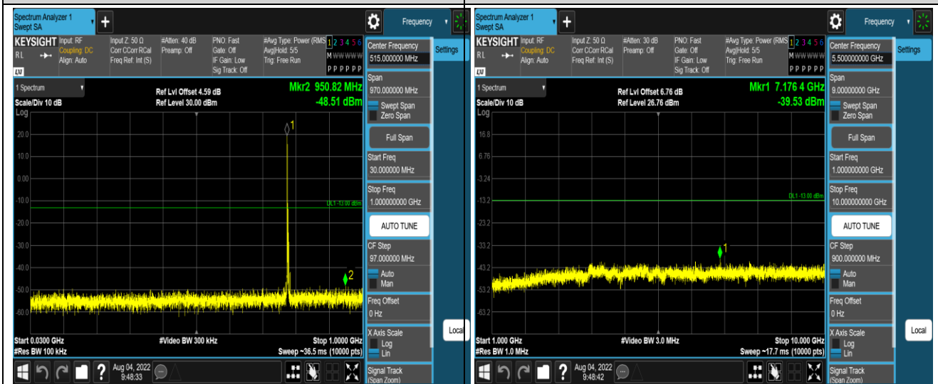
Band13-5MHz-16QAM-23230-1RB#0-Range1:30~10000MHz
