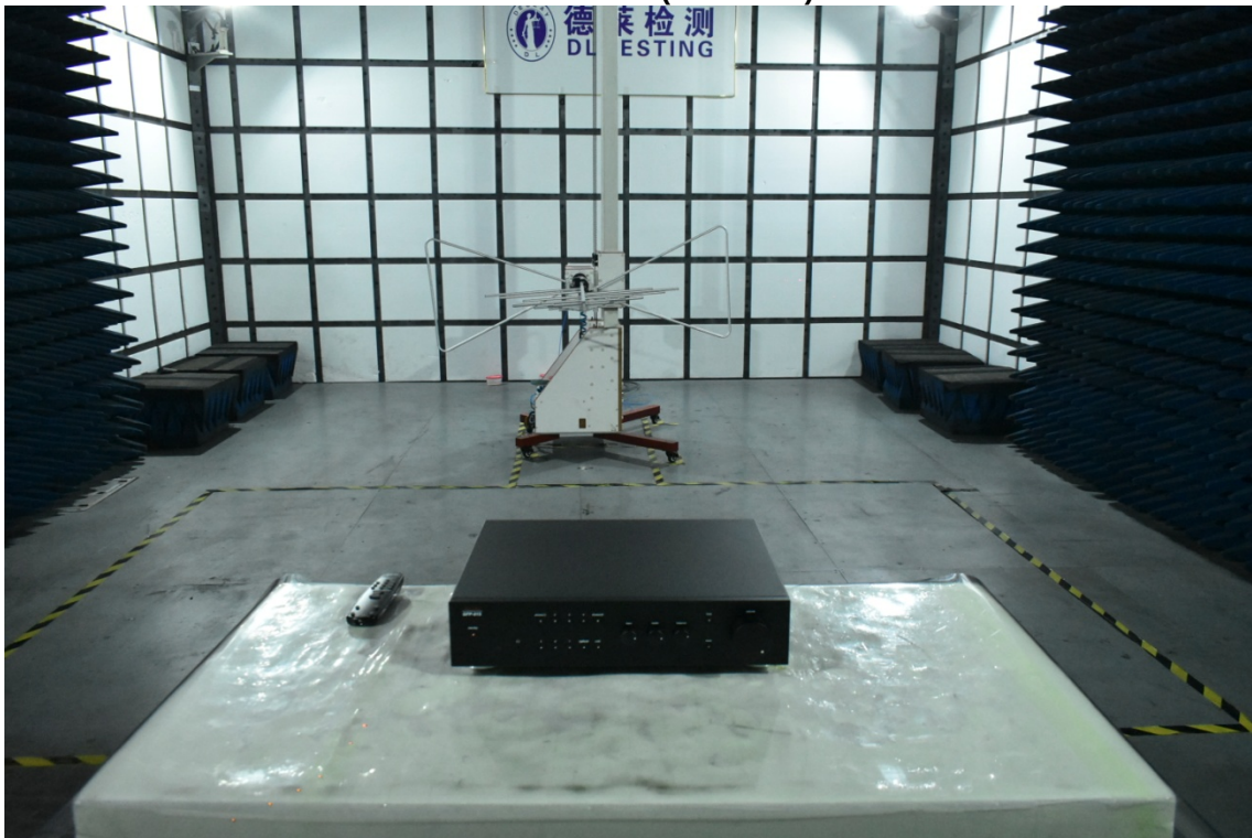
RadiatedEmission(Below 1G)
