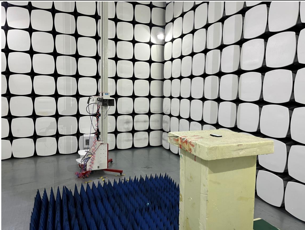
Above 1G Test setup
