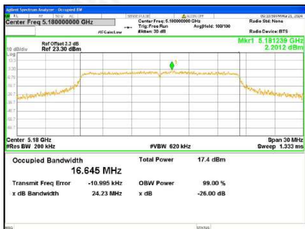
802.11a U-NII-1 Low channel
