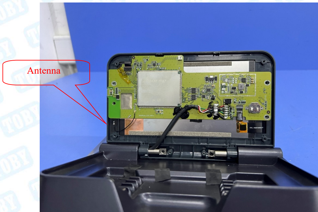
Photo 13 Internal of PCB
