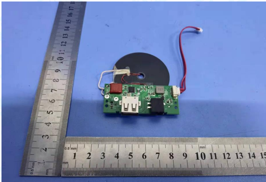
Photo 14 Appearance of PCB
