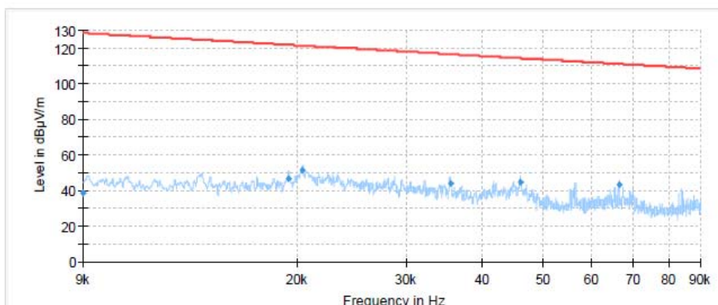
Radiates Emission from 9kHz to 90kHz
