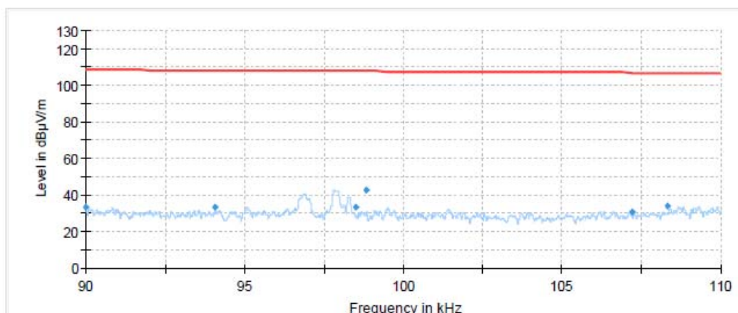
Radiates Emission from 90kHz to 110kHz
