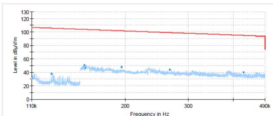
Radiates Emission from 110kHz to 490kHz
