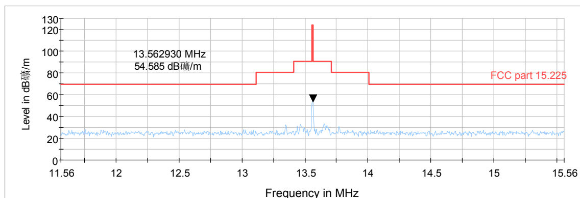
Radiates Emission from 11.56MHz to 15.56MHz
