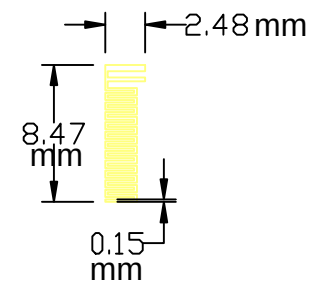
MP200 Bluetooth Antenna
