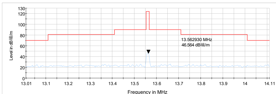
Radiates Emission from 13.01MHz to 14.11MHz
