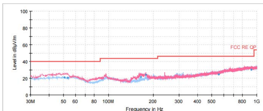
Radiated Emission from 30MHz to 1GHz
