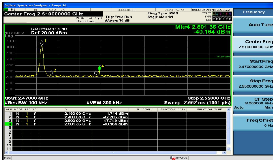
High Band Edge Plot on Channel 39
