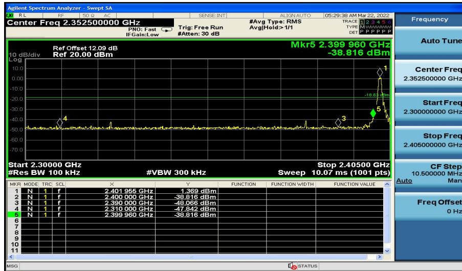
Low Band Edge Plot on Channel 00
