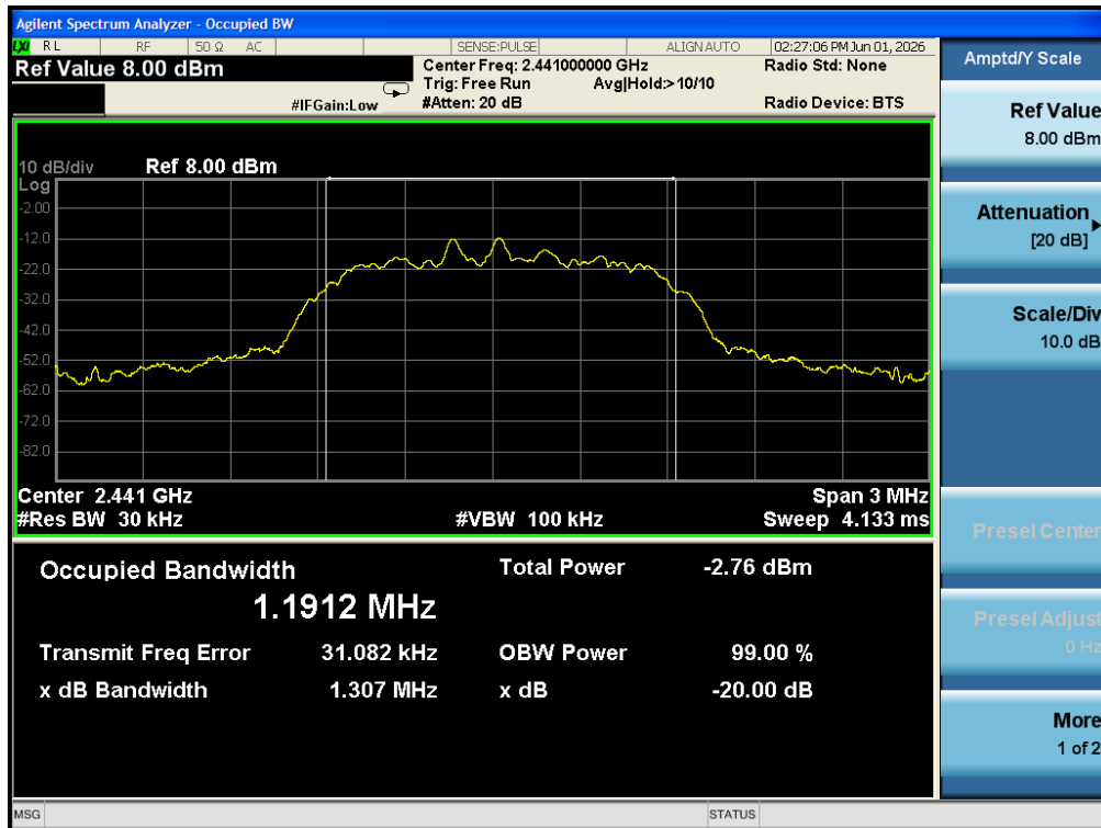
Channel 2441MHz
