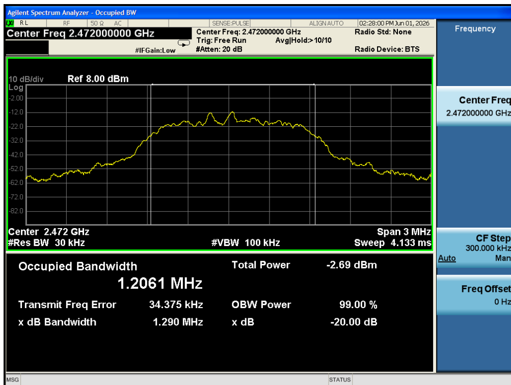
Channel 2472MHz
