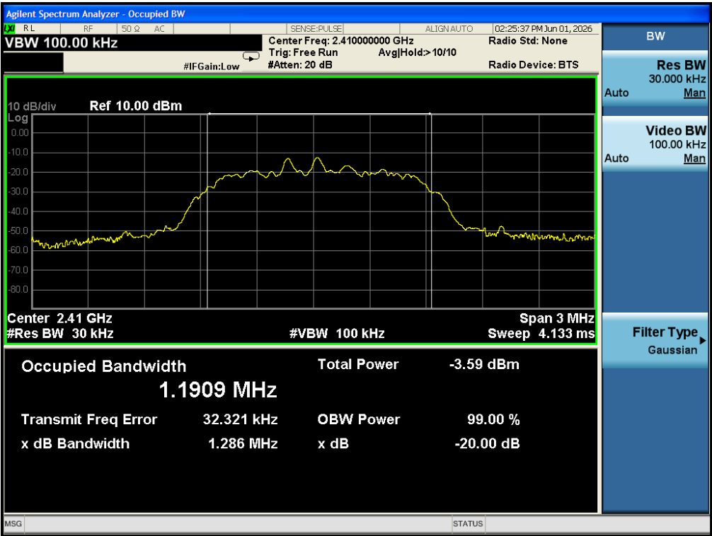
Channel 2410MHz
