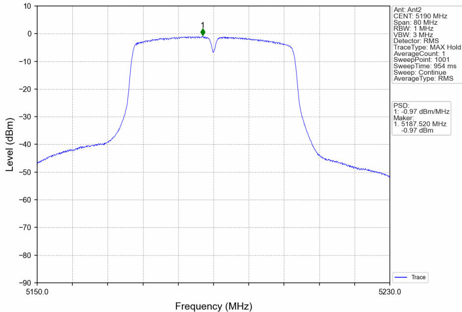
802.11ac(VHT40)_LCH_5190MHz_MIMO_NTNV
