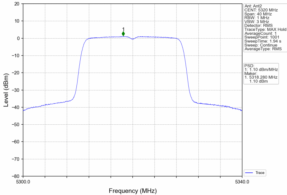
802.11ac(VHT20)_HCH_5320MHz_MIMO_NTNV
