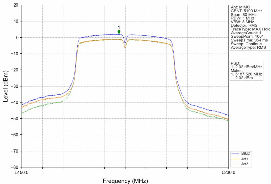
802.11ac(VHT40)_LCH_5190MHz_MIMO_NTNV
