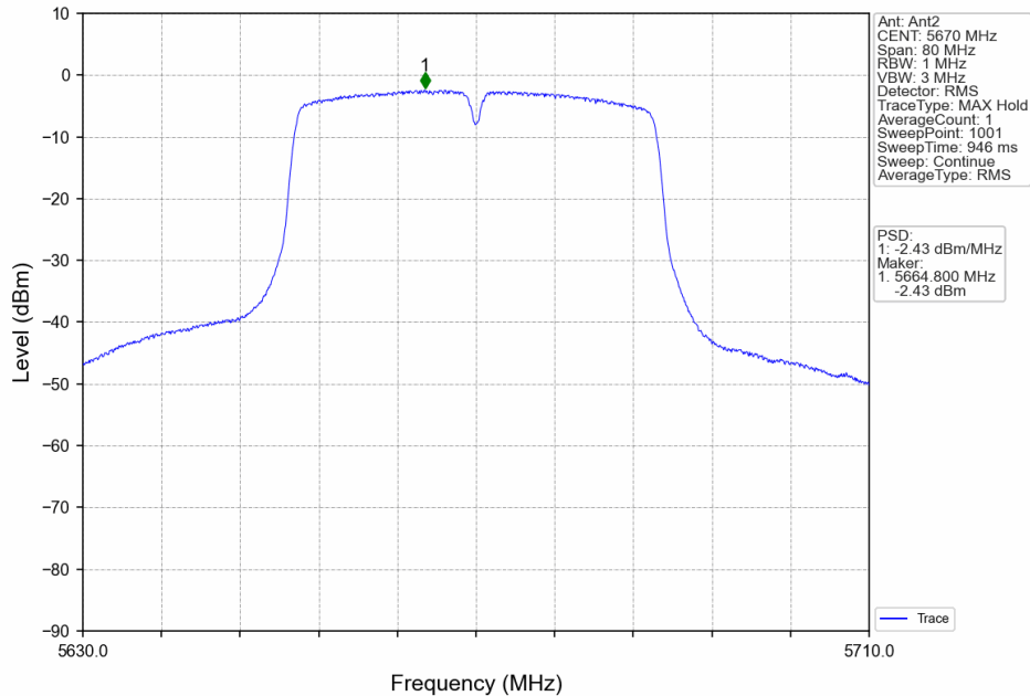
802.11n(HT40)_HCH_5670MHz_MIMO_NTNV
