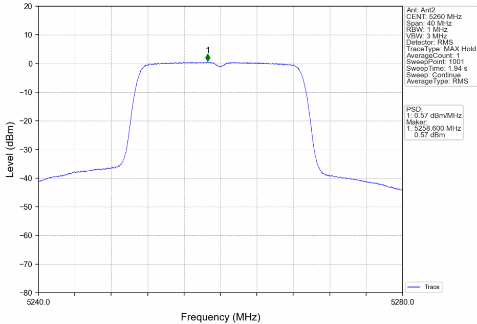
802.11ac(VHT20)_LCH_5260MHz_MIMO_NTNV
