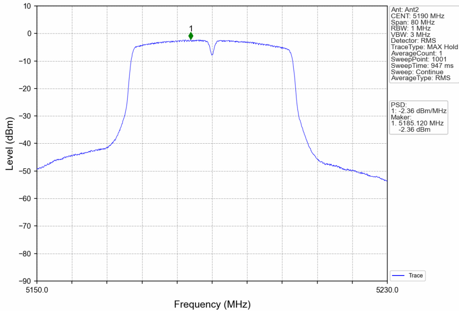
802.11n(HT40)_LCH_5190MHz_MIMO_NTNV
