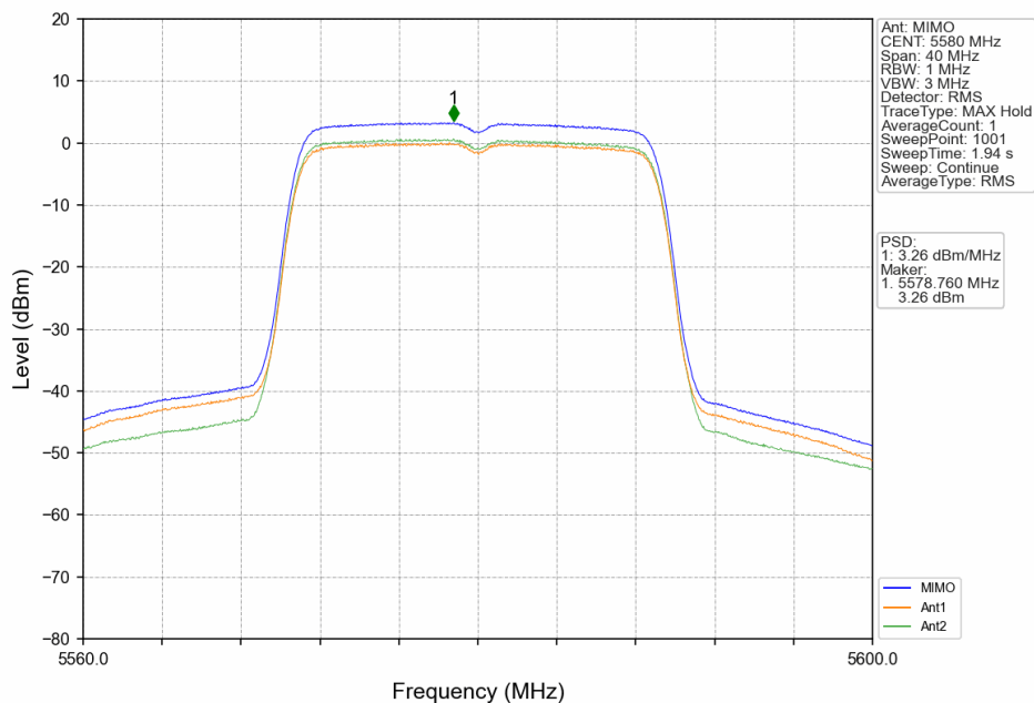
802.11ac(VHT20)_MCH_5580MHz_MIMO_NTNV
