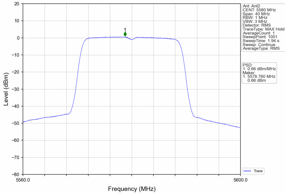
802.11ac(VHT20)_MCH_5580MHz_MIMO_NTNV
