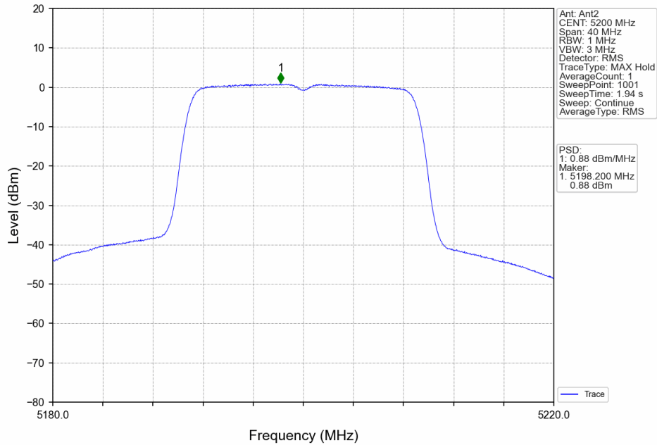
802.11ac(VHT20)_MCH_5200MHz_MIMO_NTNV
