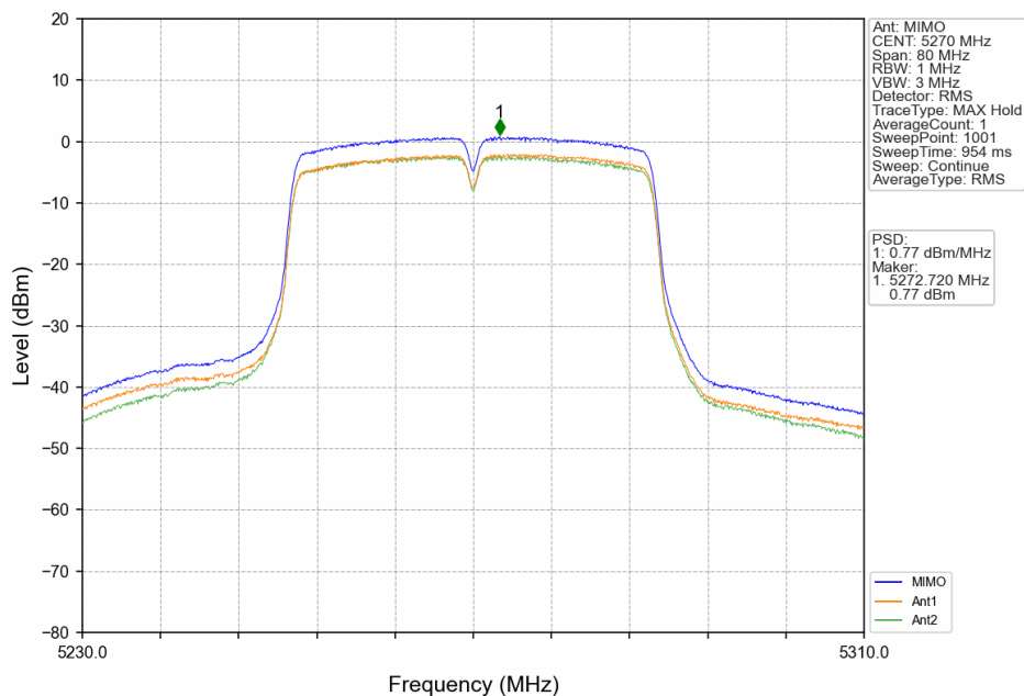
802.11ac(VHT40)_LCH_5270MHz_MIMO_NTNV
