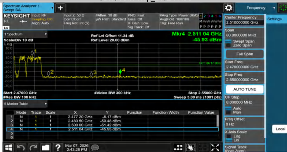
3DH5-Ant1-Hop_2480-PASS
