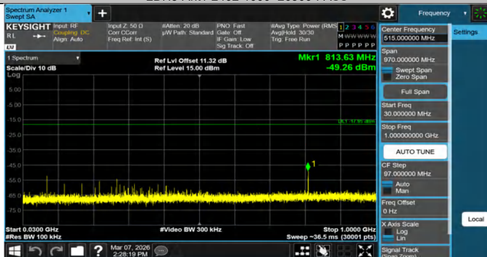
2DH5-Ant1-2441-30~1000-PASS
