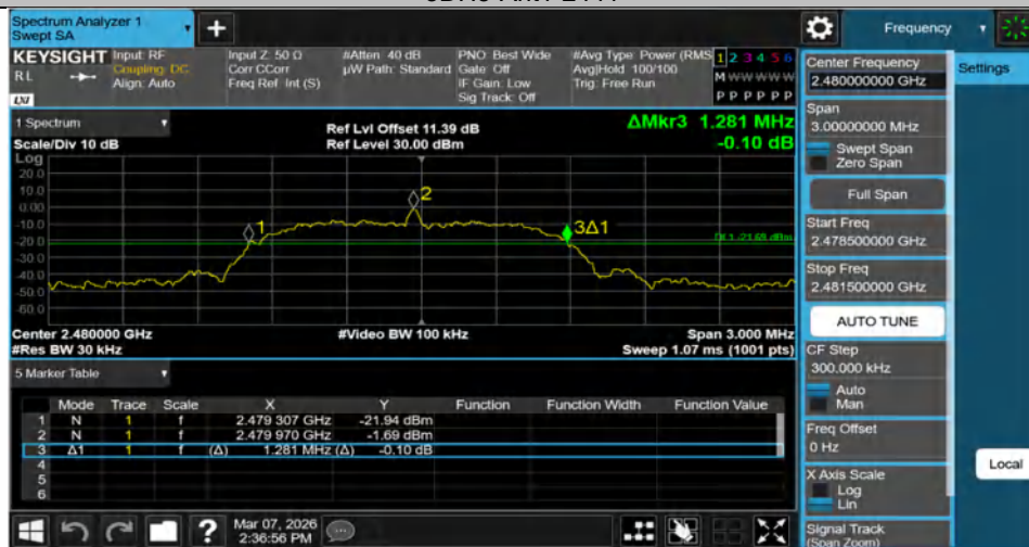
3DH5-Ant1-2480
