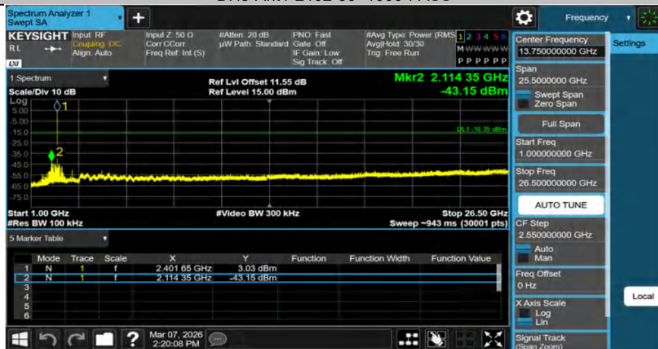
DH5-Ant1-2402-1000~26500-PASS
