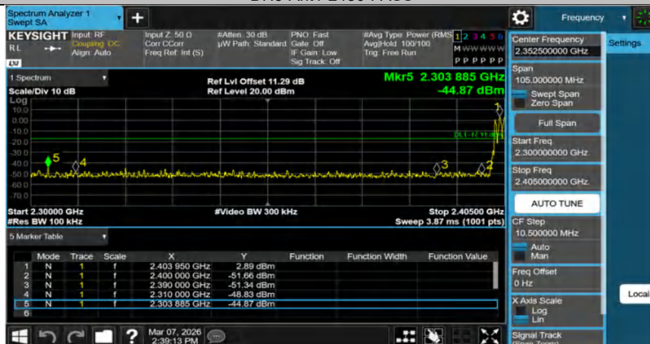
DH5-Ant1-Hop_2402-PASS
