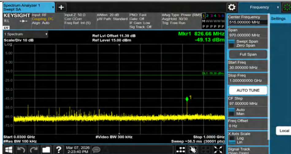
DH5-Ant1-2480-30~1000-PASS
