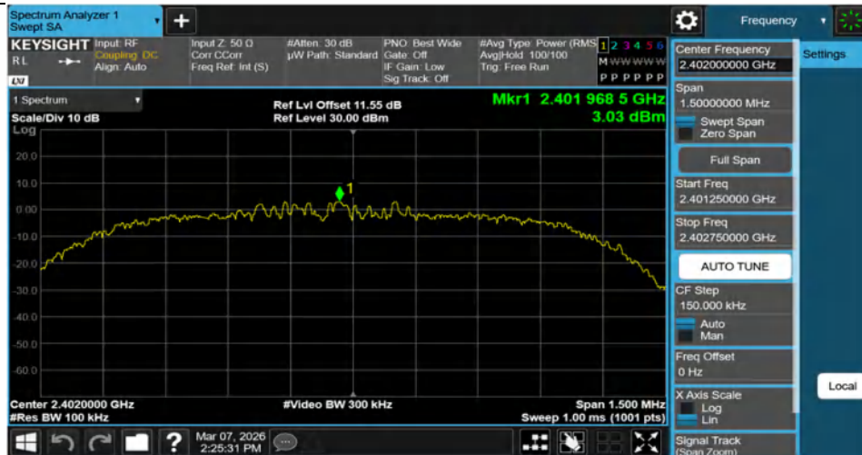
2DH5-Ant1-2402-PASS
