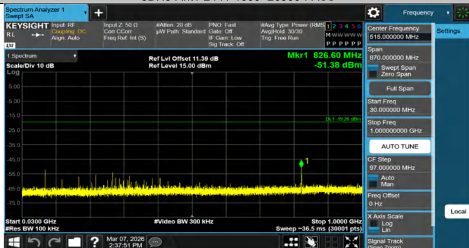
3DH5-Ant1-2480-30~1000-PASS
