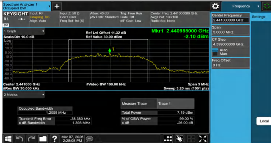
2DH5-Ant1-2441
