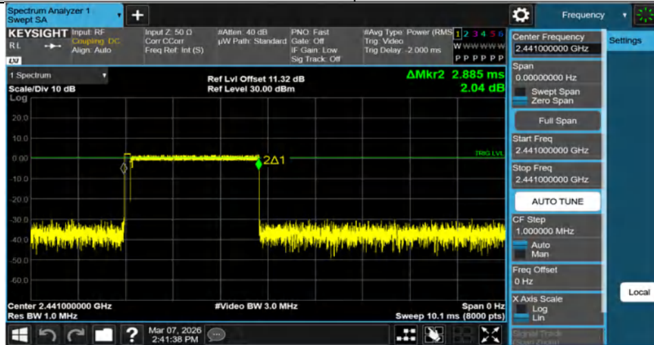
2DH5-Ant1-Hop-PASS
