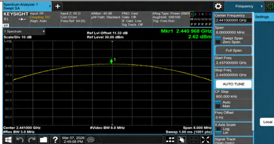
2DH5-Ant1-2441-PASS
