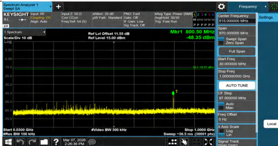
2DH5-Ant1-2402-30~1000-PASS
