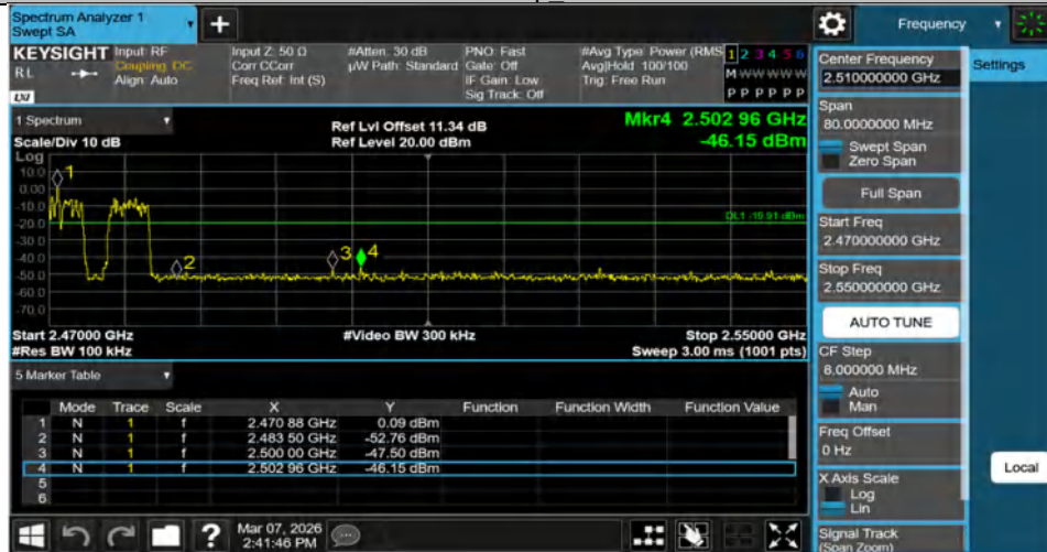
2DH5-Ant1-Hop_2480-PASS
