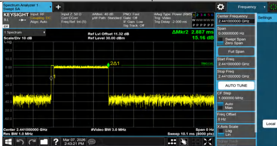
3DH5-Ant1-Hop-PASS
