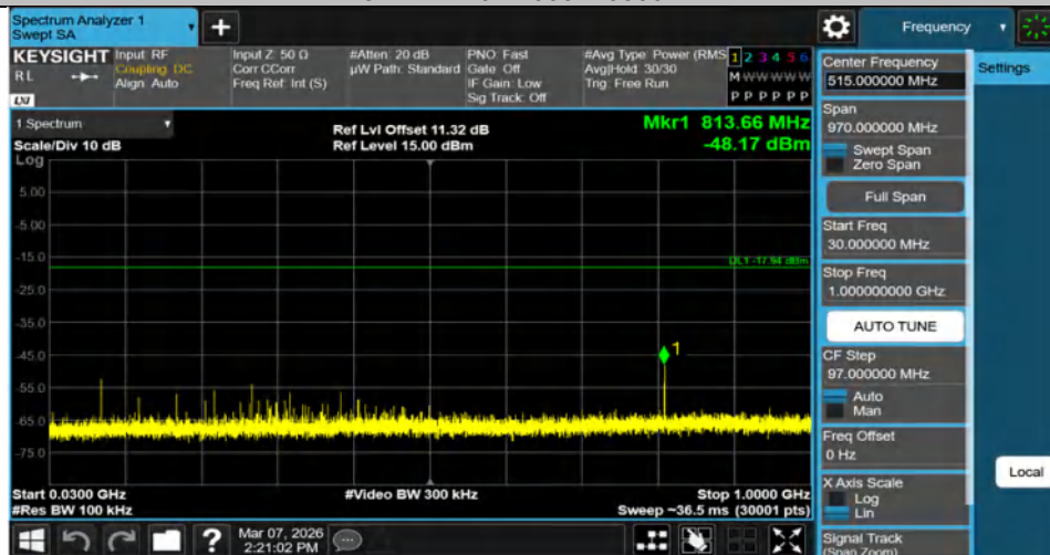
DH5-Ant1-2441-30~1000-PASS
