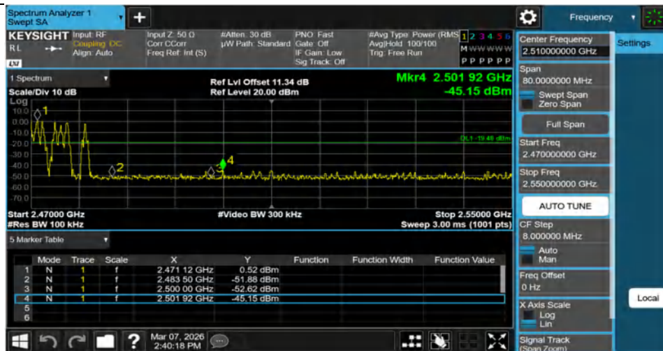
DH5-Ant1-Hop 2480-PASS
