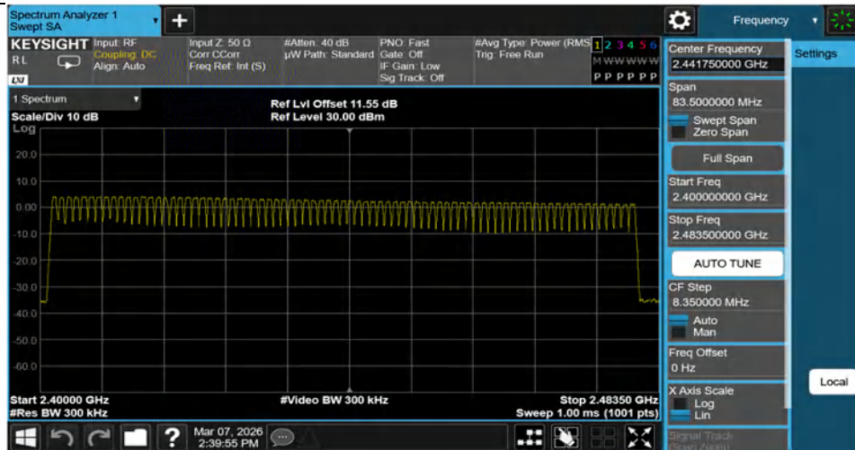
DH5-Ant1-Hop-PASS
