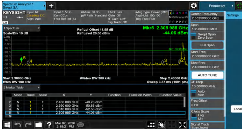
DH5-Ant1-2402-PASS
