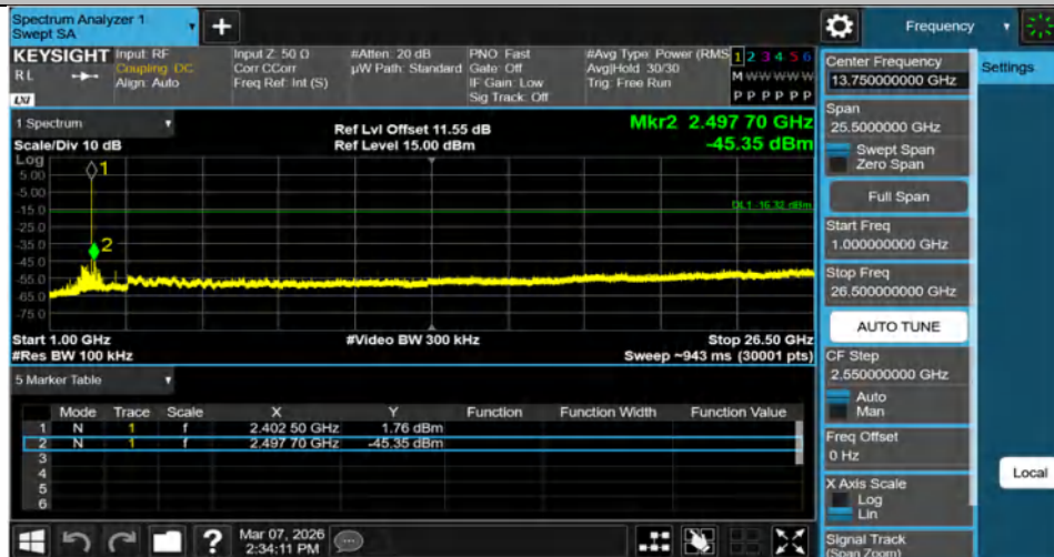
3DH5-Ant1-2402-1000~26500-PASS
