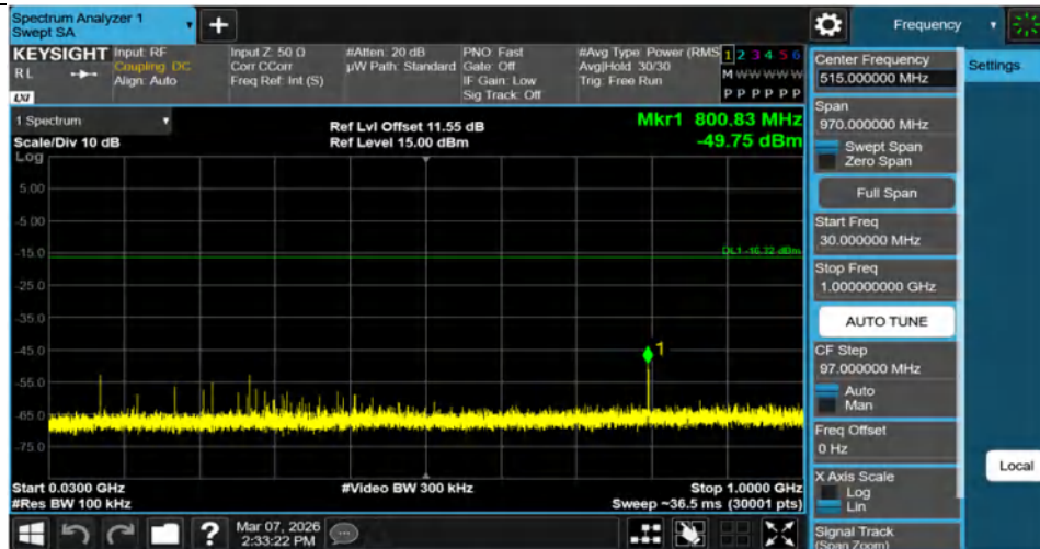
3DH5-Ant1-2402-30~1000-PASS
