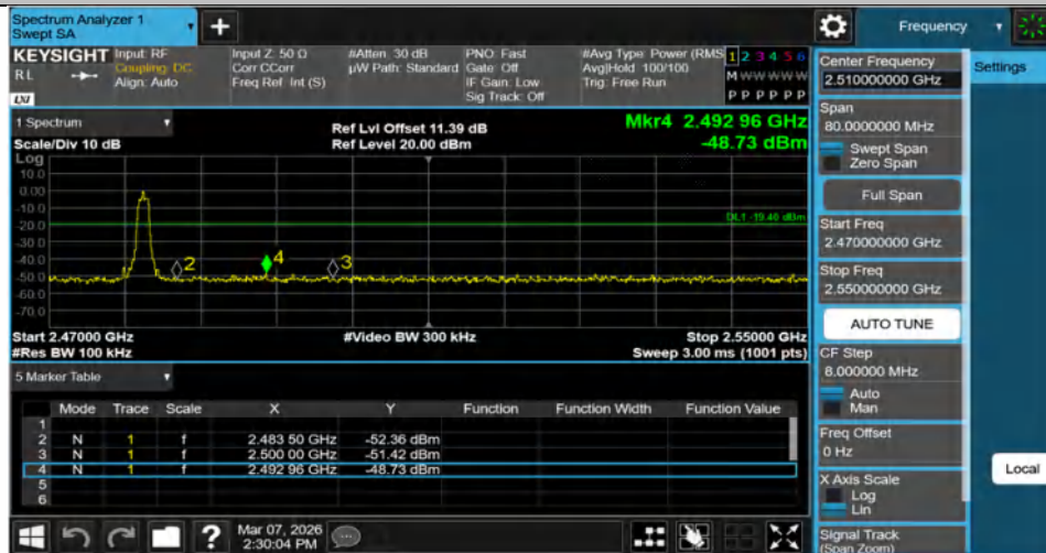
2DH5-Ant1-2480-PASS
