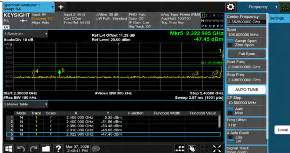
2DH5-Ant1-Hop_2402-PASS
