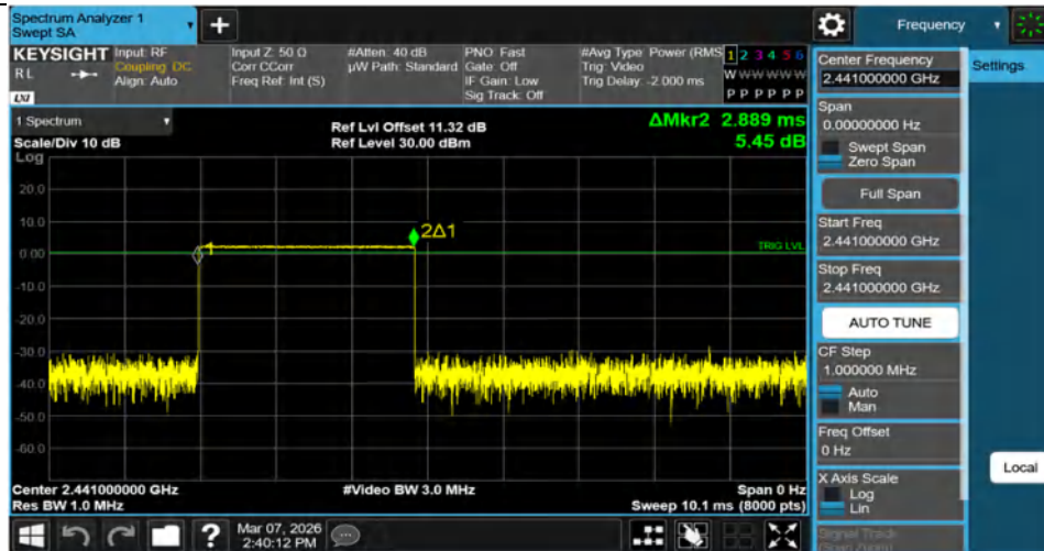
DH5-Ant1-Hop-PASS
