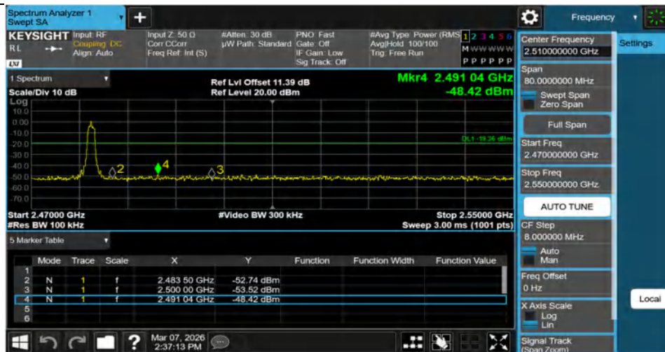
3DH5-Ant1-2480-PASS
