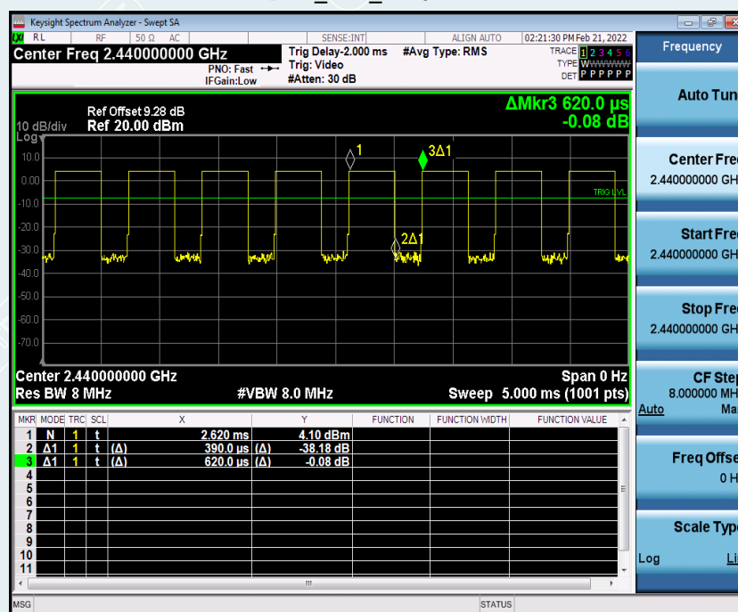
BLE_1M_2440 MHz
