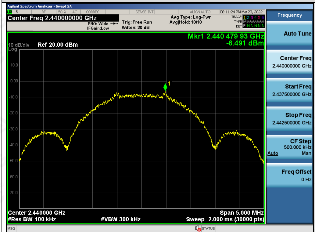
Test_Graph_GFSK_ANT1_2440_Reference Level
