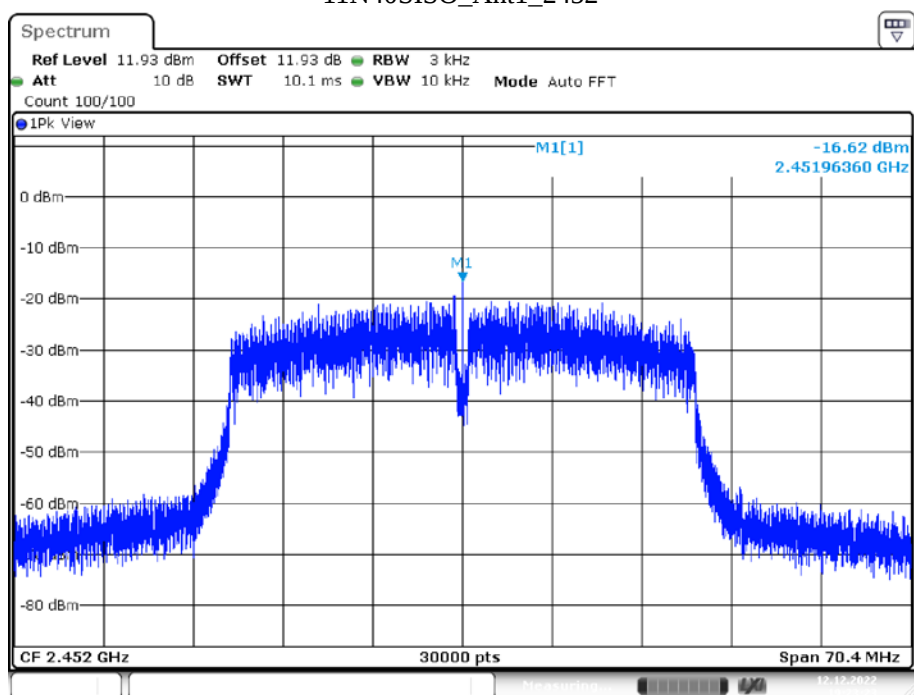
11N40SISO_Ant1_2452
