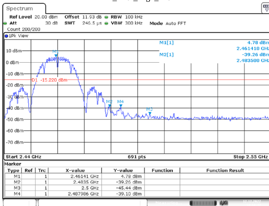
11B_Ant1_High_2462
