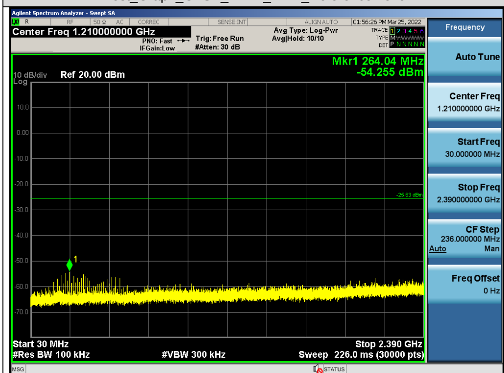
Test_Graph_GFSK_ANT1_2417_Lower Band Emissions
