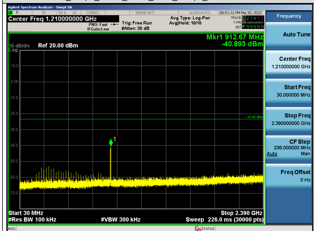
Test_Graph_GFSK_ANT1_2417_1Mbps_Lower Band Emissions
