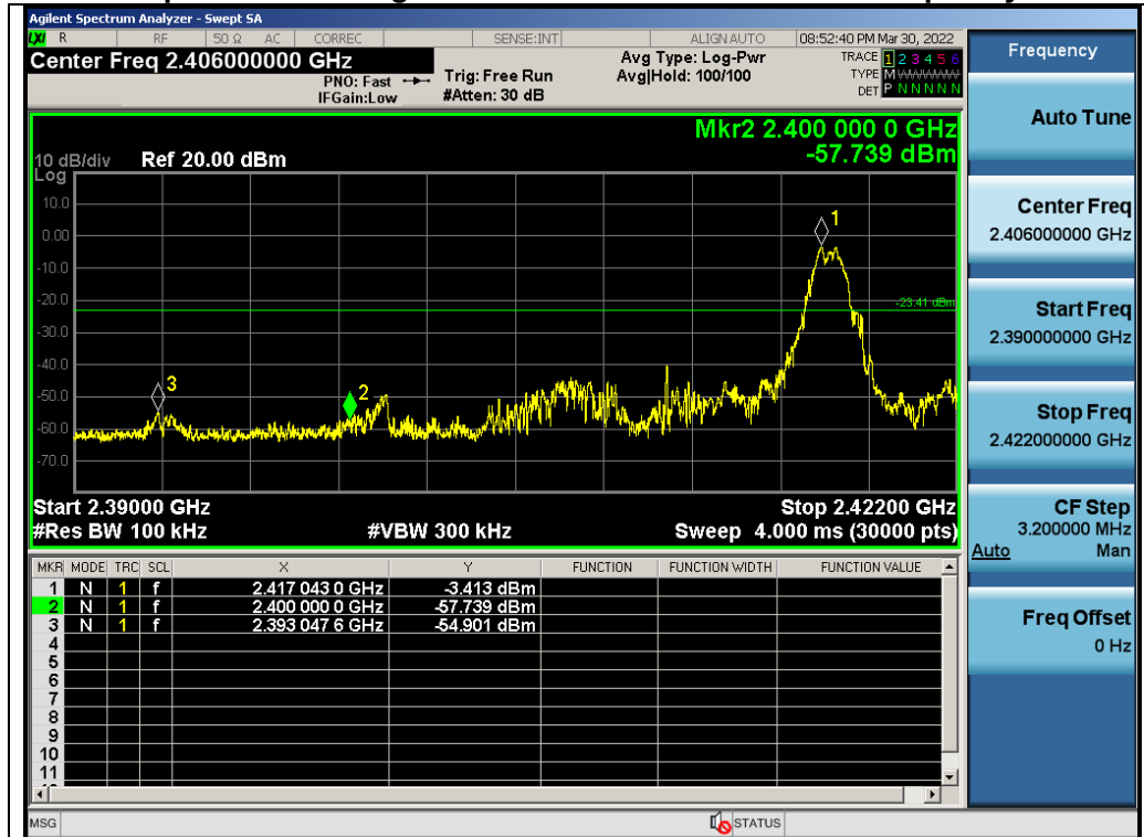
Test_Graph_GFSK_ANT1_2417_1Mbps_Lower Band Edge Emissions
