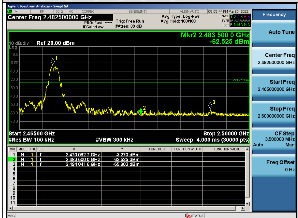
Test_Graph_GFSK_ANT1_2470_1Mbps_Higher Band Edge Emissions
