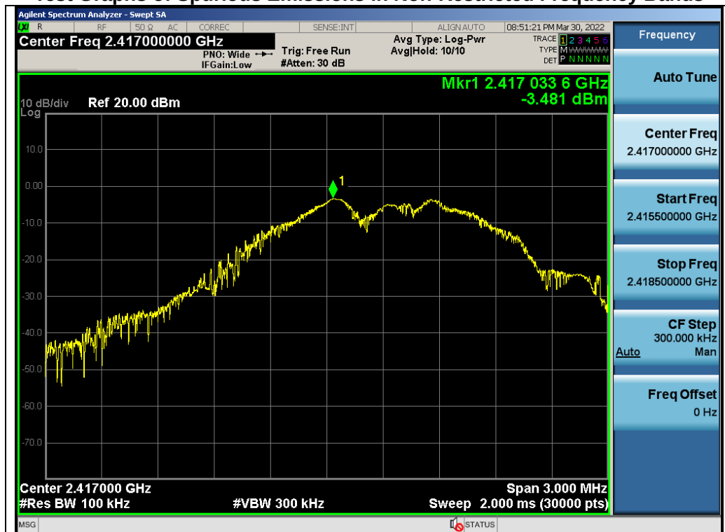
Test_Graph_GFSK_ANT1_2417_1Mbps_Reference Level
