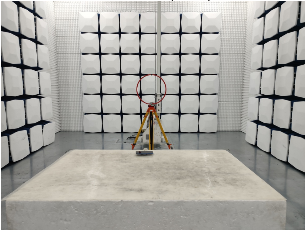
Radiated Emission (Below 30)
