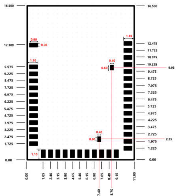
[ PCB FOOTPRINT ]
