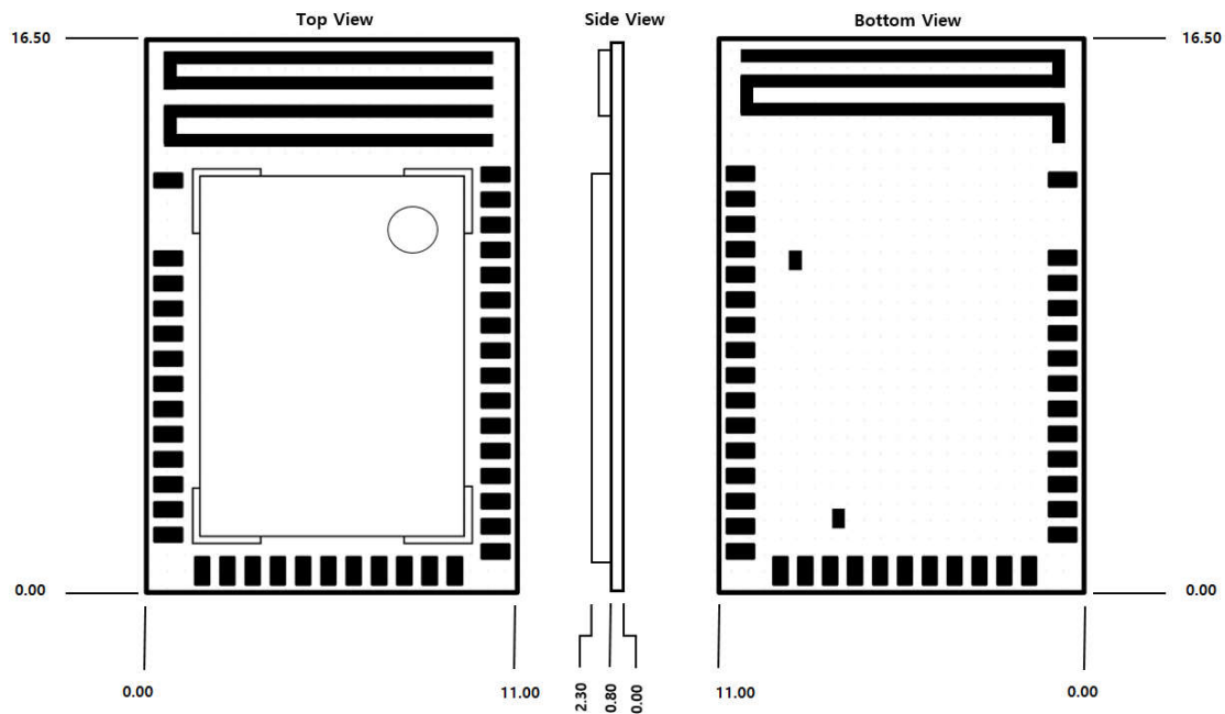
[ DIMENSIONS ]
