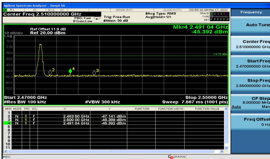
High Band Edge Plot on Channel 39
