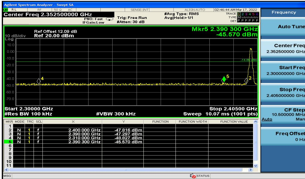
Low Band Edge Plot on Channel 00
