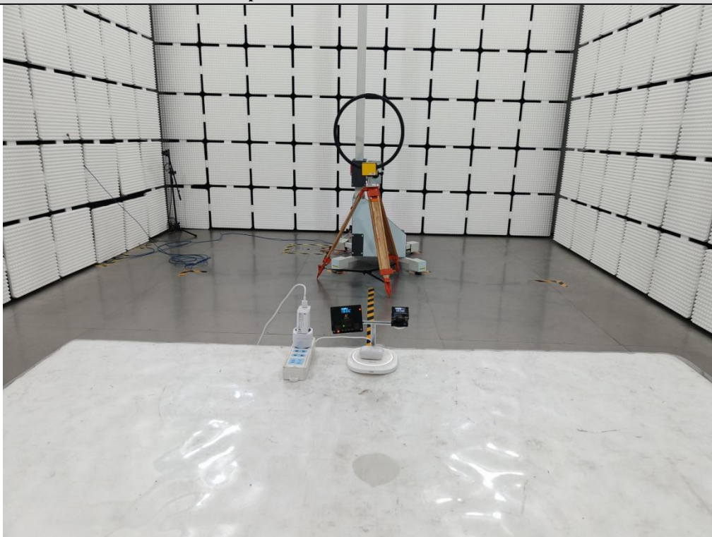
Radiated Spurious Emission Below 9kHz~30MHz
