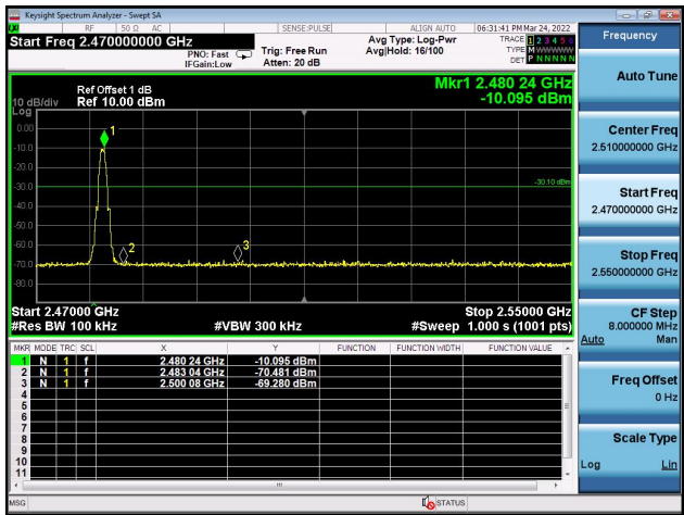
Right bandedge
