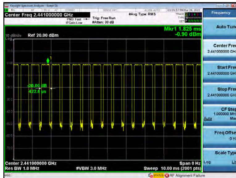
Test Plots GFSK DH1 2441MHZ
