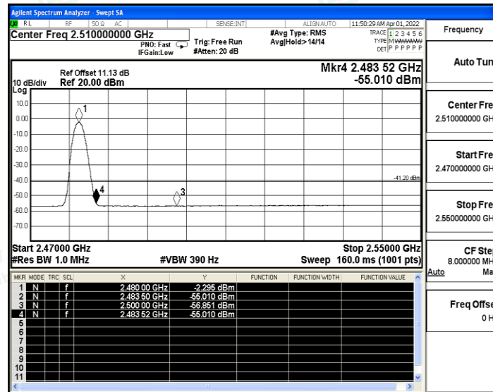
2DH5_Ant1_High_2480_Peak
