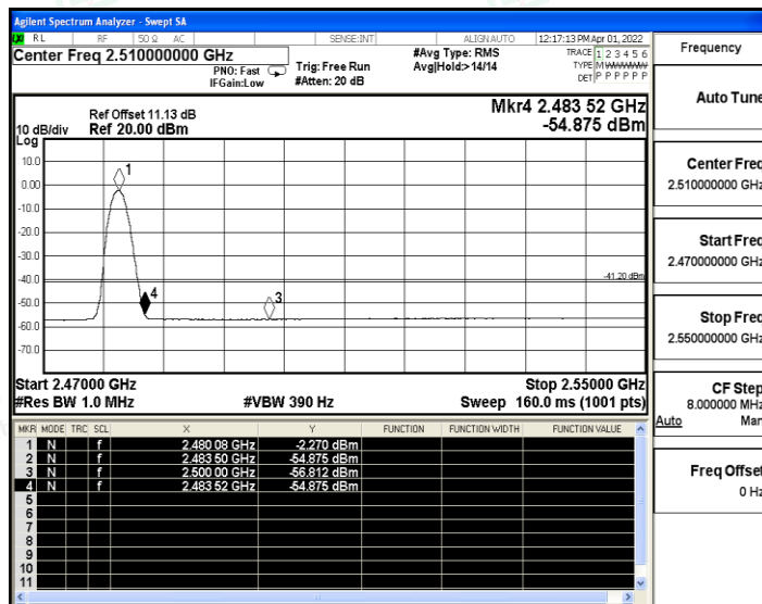
3DH5_Ant1_High_2480_Peak
