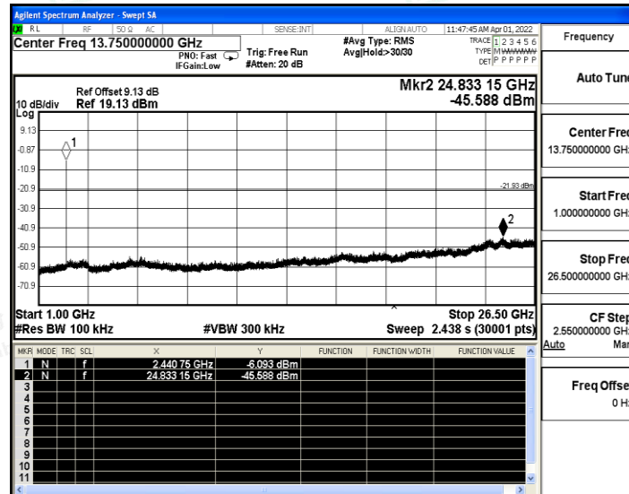
2DH5_Ant1_2480_0~Reference
