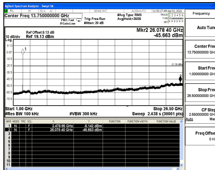
3DH5_Ant1_2402_0~Reference
