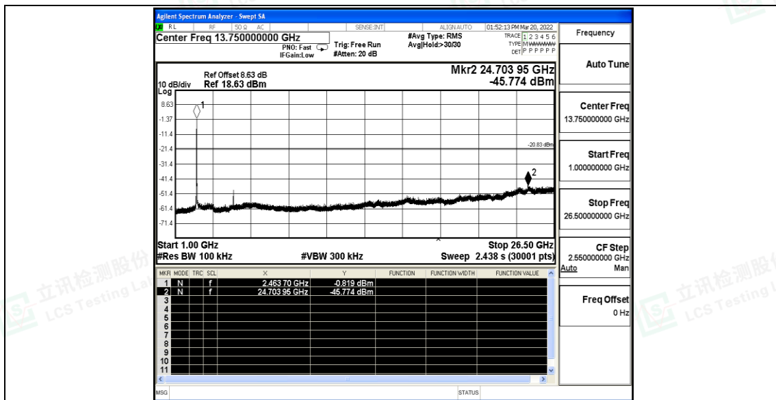
11AX20SISO_Ant A_2412_0~Reference
