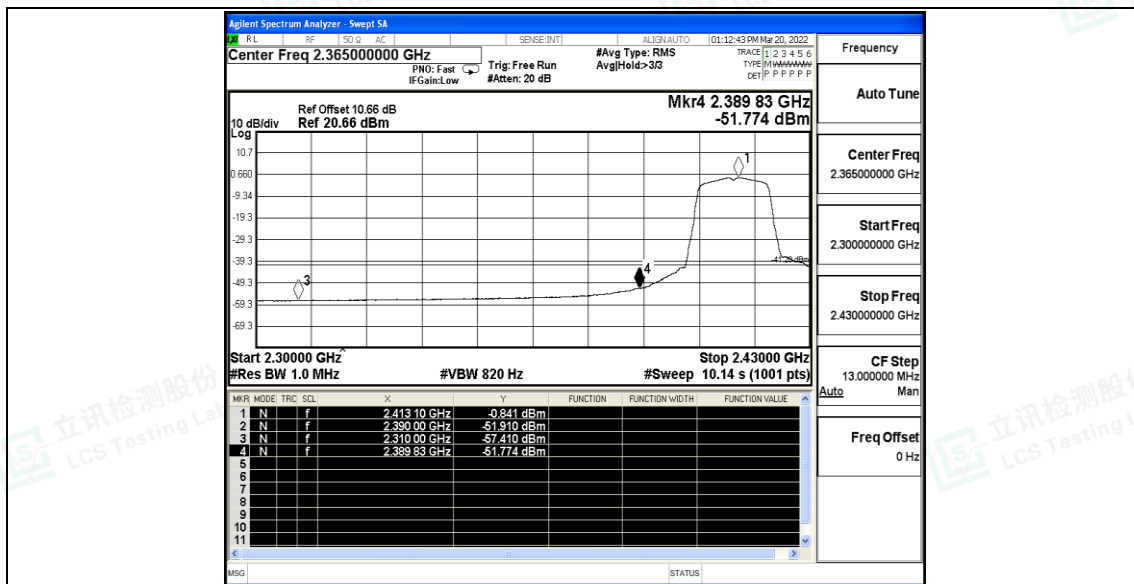
11G_Ant A_Low_2412_Peak
