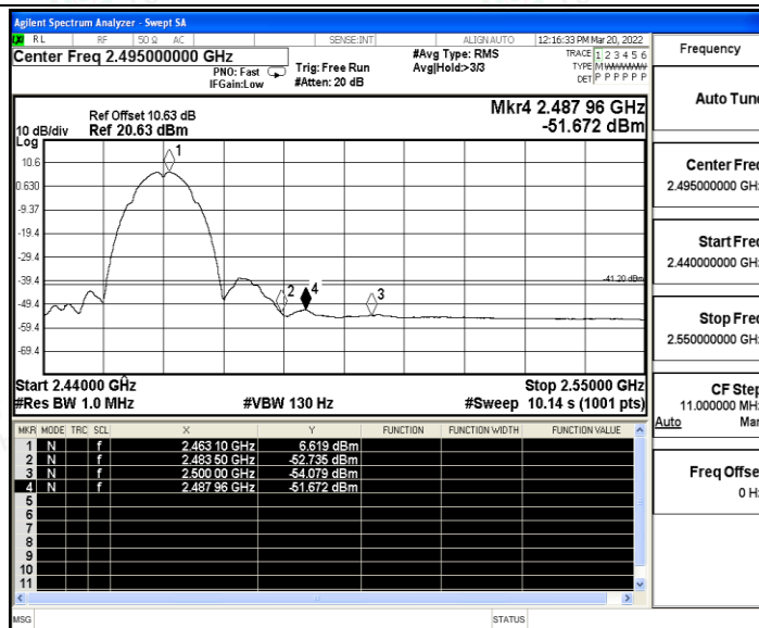
11B_Ant A_High_2462_Peak
