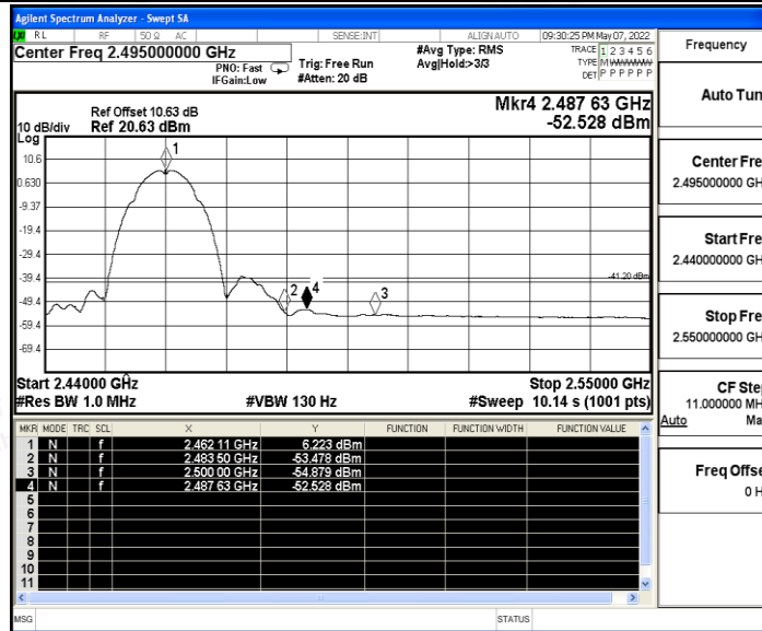
11B_Ant B_High_2462_Peak
