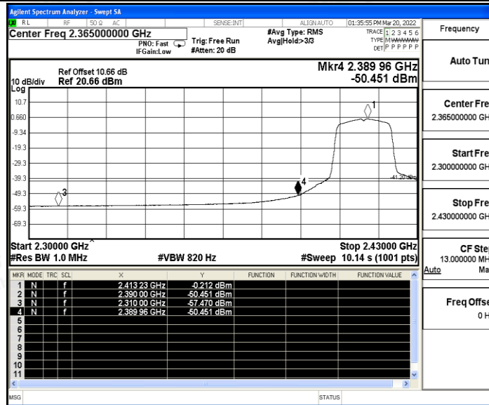
11N20SISO_Ant A_Low_2412_Peak
