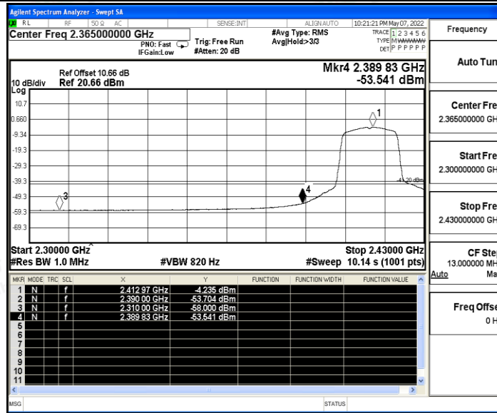
11N20SISO_Ant B_Low_2412_Peak
