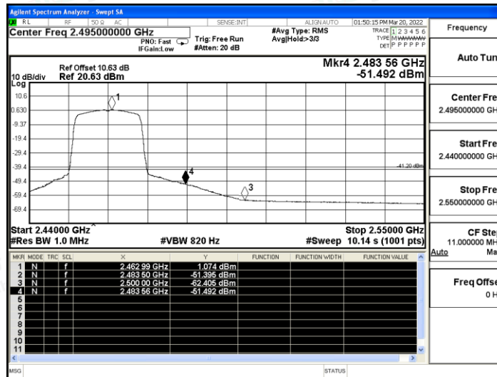
11N20SISO_Ant A_High_2462_Peak
