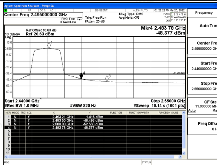
11G_Ant A_High_2462_Peak
