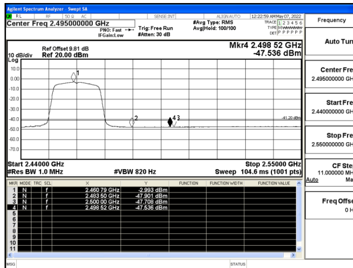
11AX20SISO_Ant A_High_2462_Peak
