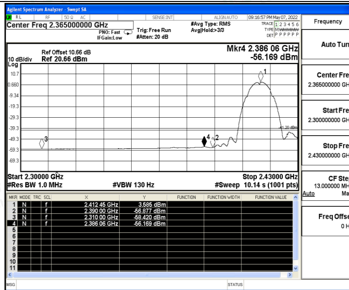
11B_Ant B_Low_2412_Peak
