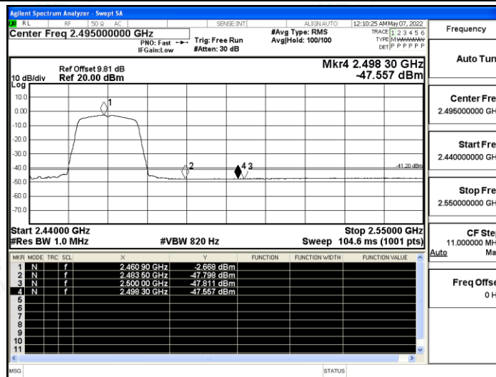
11N20SISO_Ant B_High_2462_Peak
