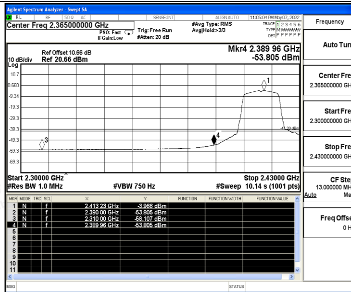
11G_Ant B_Low_2412_Peak
