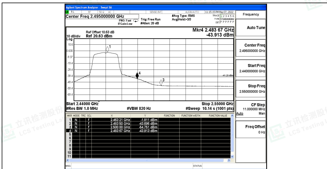
11G_Ant B_High_2462_Peak
