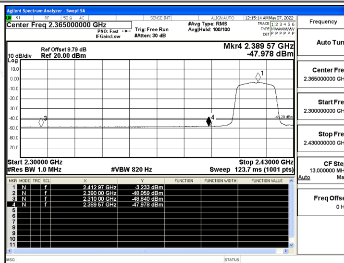
11AX20SISO_Ant A_Low_2412_Peak
